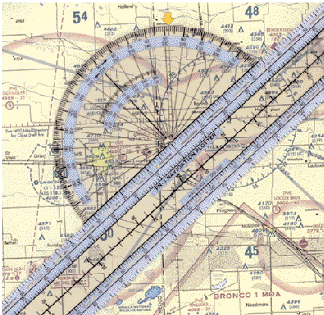
Figure 11-5. Navigational plotter.
