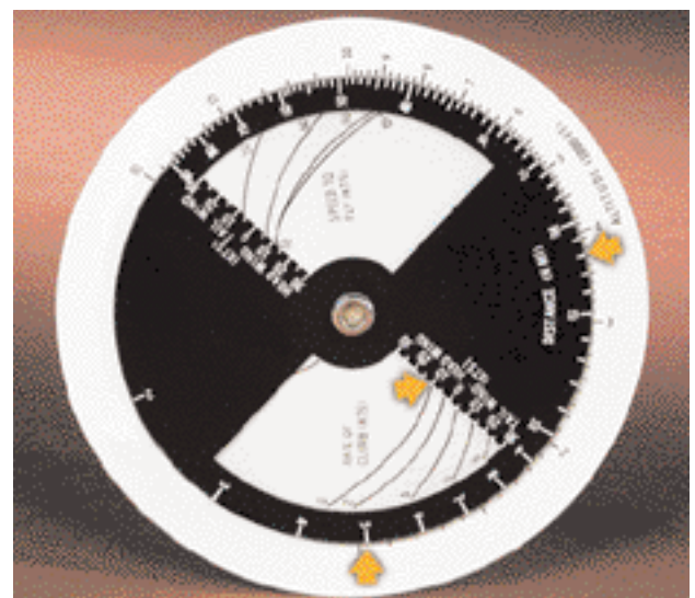
Figure 11-3. Circular glide calculator.
