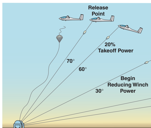
Figure 7-17. Winch procedures.
