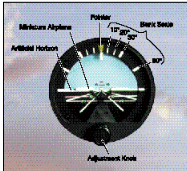
Figure 4-25. Attitude Indicator.
