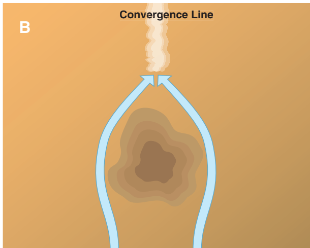
Figure 9-32. Convergence induced by flow around topography.
