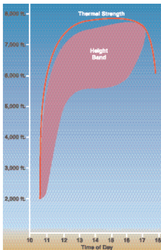
Figure 11-12. Thermal height and height band (shaded) vs. time of day.
