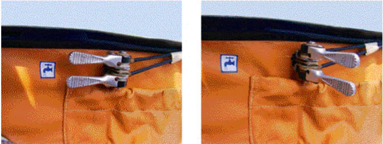
Figure 5-20. Water ballast drain valve handles.
