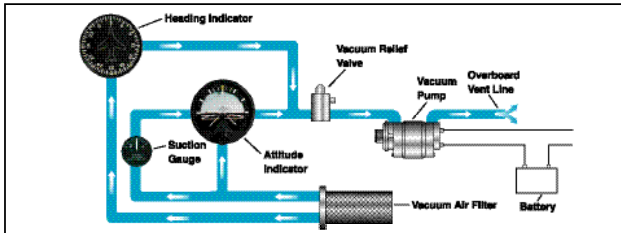
Figure 4-23. Electric powered gyro system.
