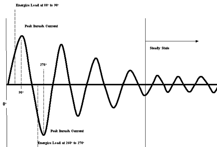
Figure 1 Inrush Current Limit Measurements
