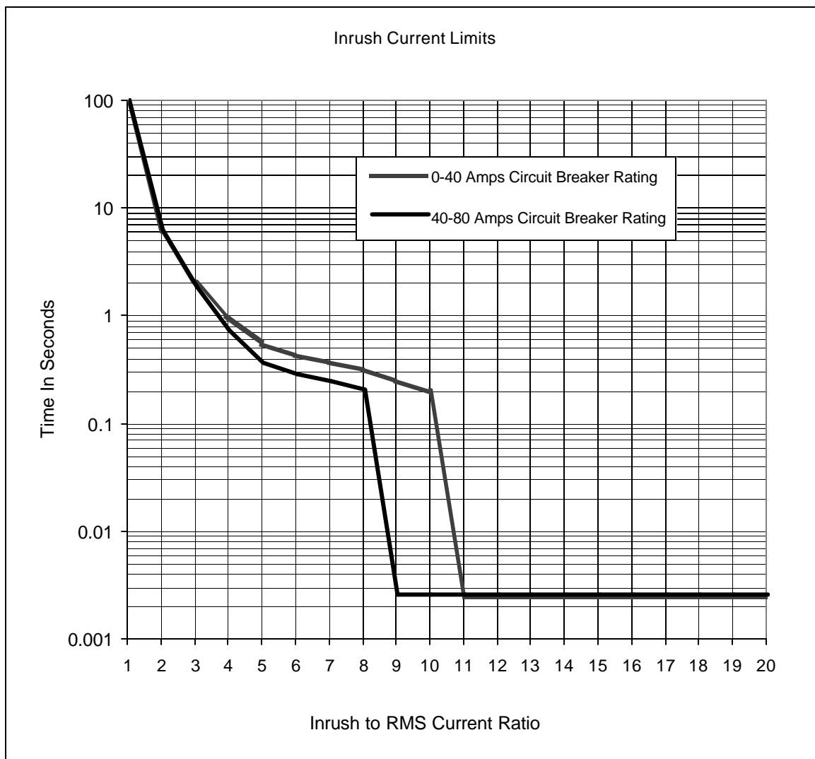
Figure 2 Inrush Current Limit Ratios
