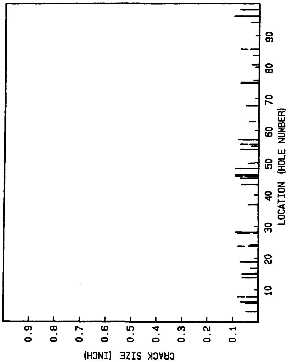
FIGURE 22. SIZE DISTRIBUTION WHEN LARGEST CRACK IS 0.1 INCH
