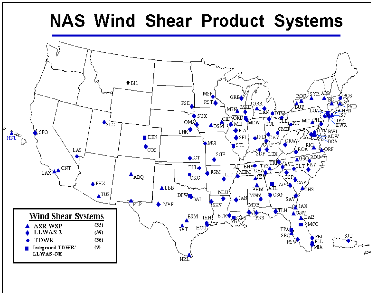
FIG 7-1-14 NAS Wind Shear Product Systems
