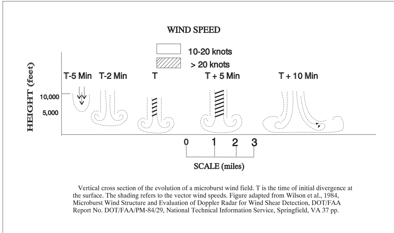
FIG 7-1-12 Evolution of a Microburst
