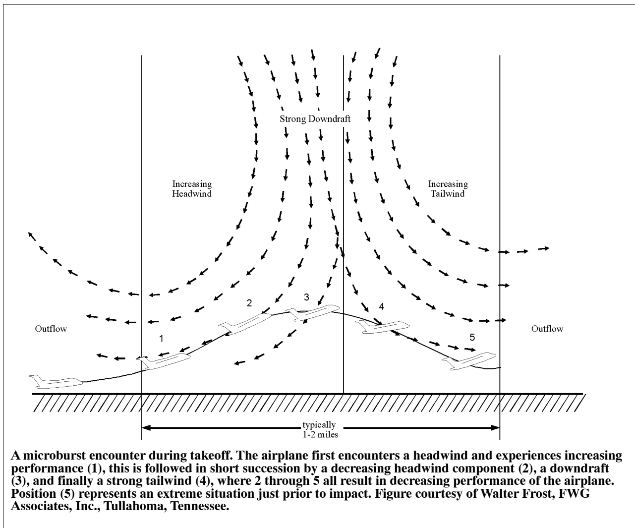
FIG 7-1-13 Microburst Encounter During Takeoff
