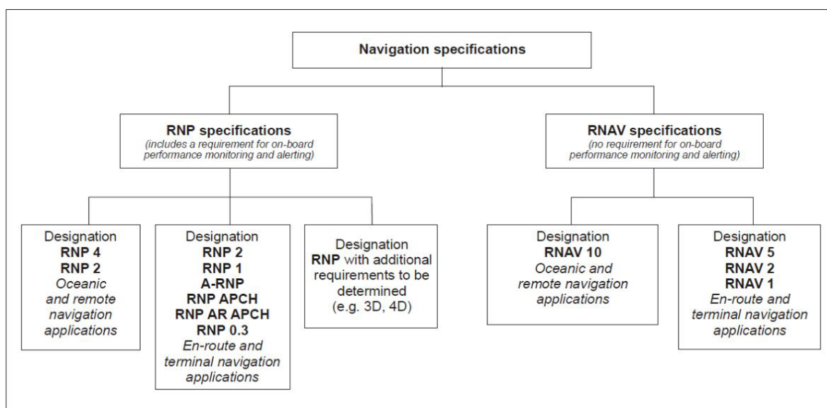
FIG 1-2-1 Navigation Specifications
