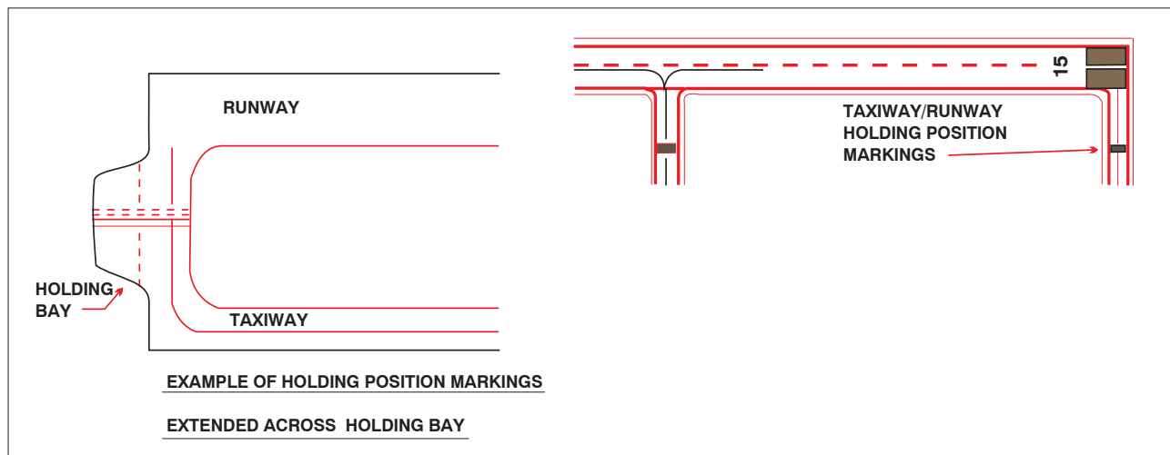
FIG 2-3-13 Runway Holding Position Markings on Taxiway
