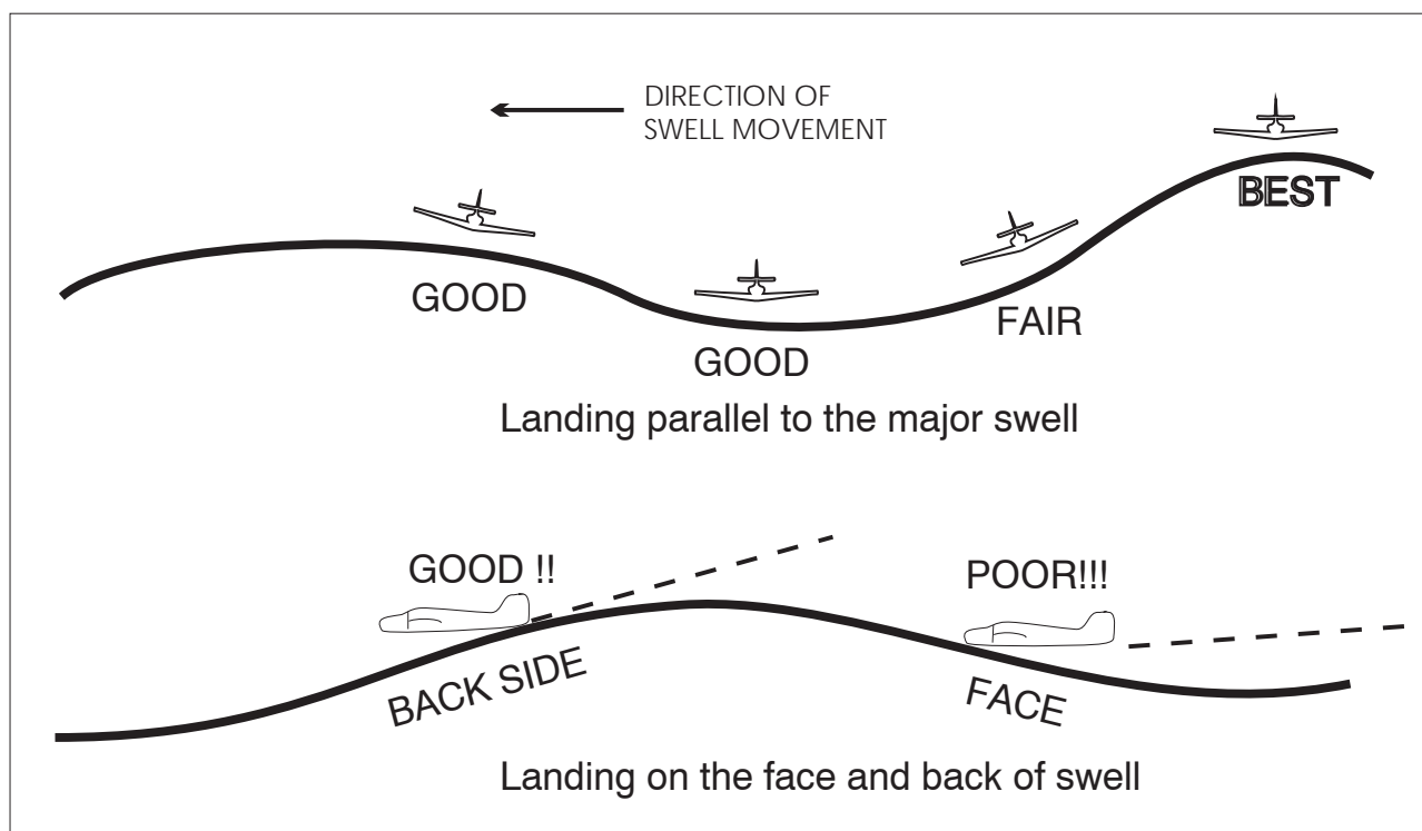
FIG 6-3-5 Wind-Swell-Ditch Heading
