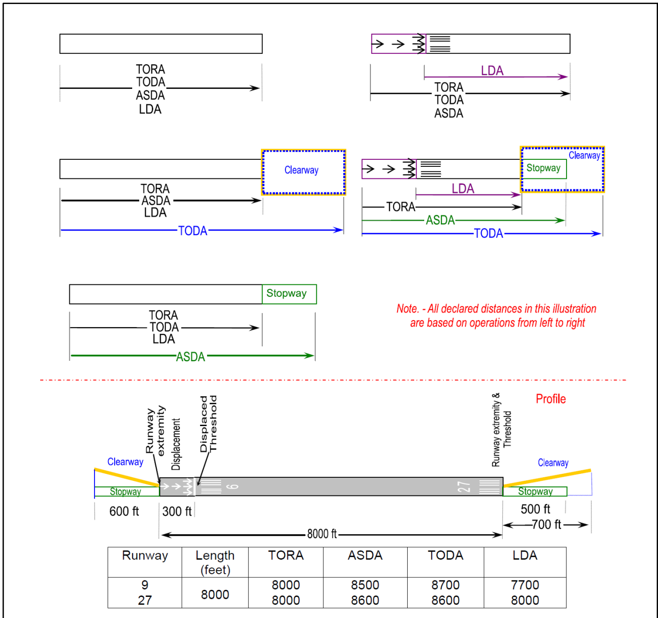
FIG 4-3-5 Declared Distances with Full-Standard Runway Safety Areas, Runway Object Free Areas, and Runway Protection Zones
