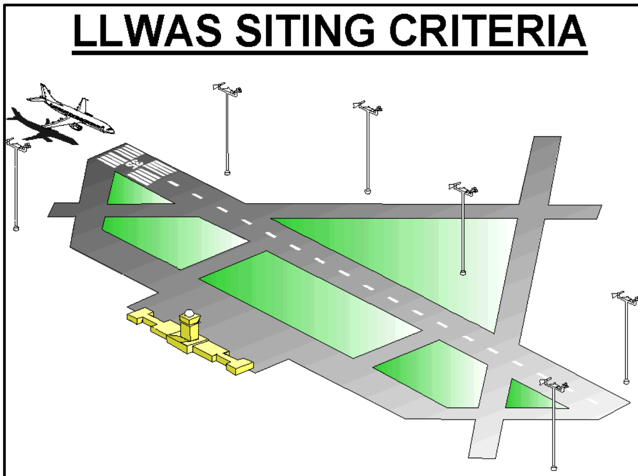
FIG 7-1-15 LLWAS Siting Criteria
