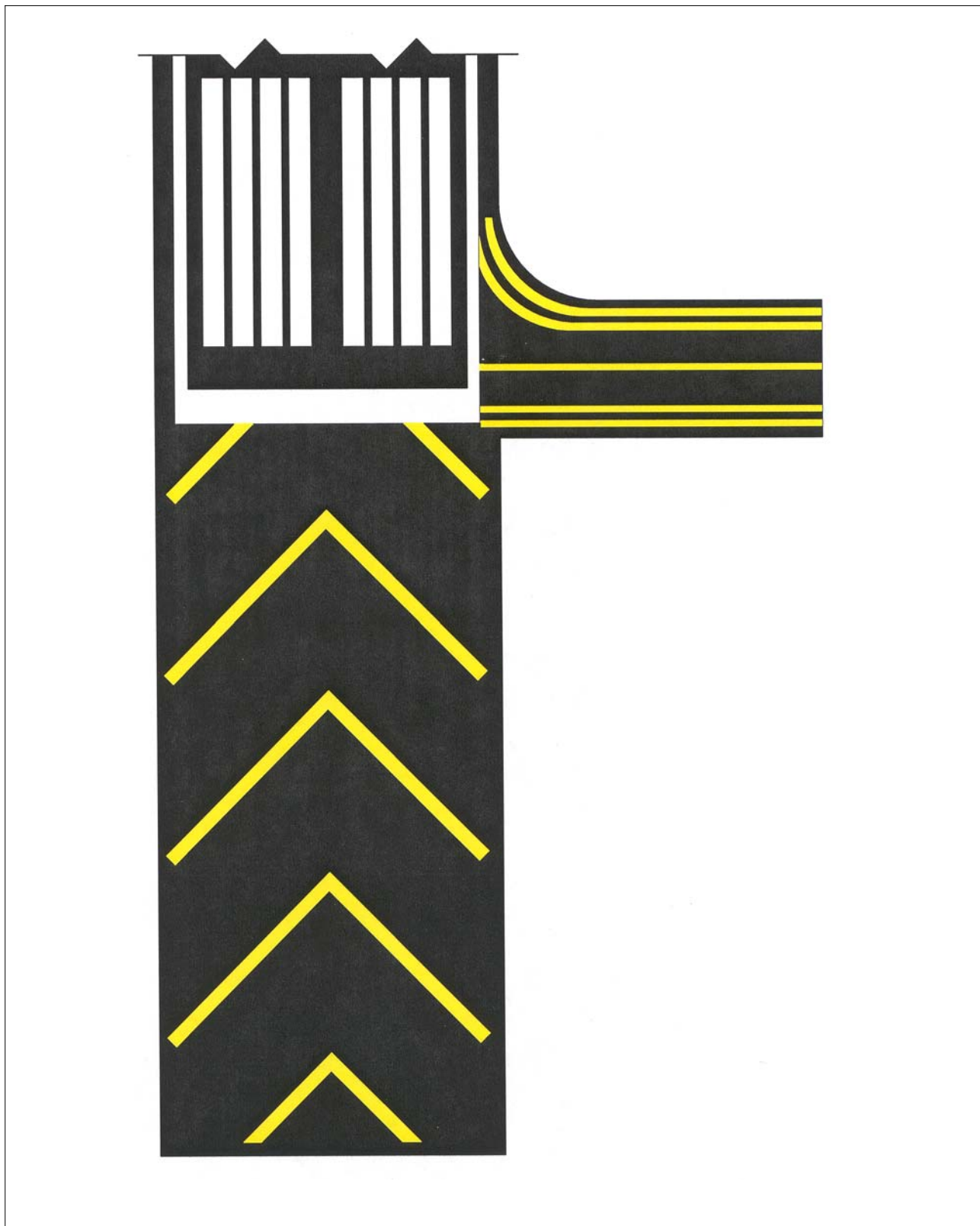
FIG 2-3-7 Markings for Blast Pads and Stopways
