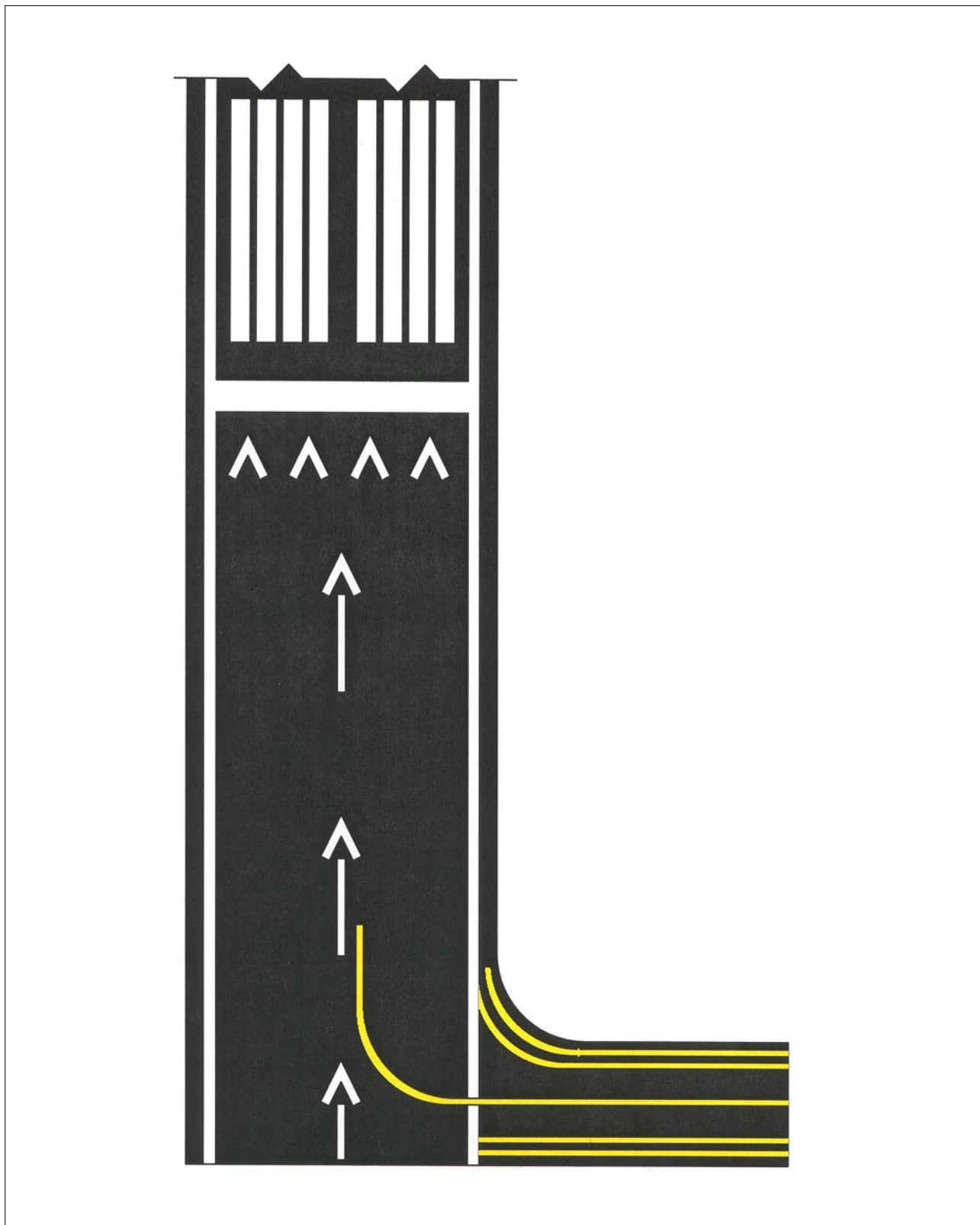
FIG 2-3-4 Displaced Threshold Markings
