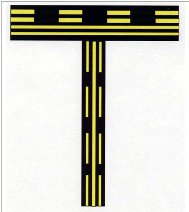
FIG 2-3-9 Dashed Markings
