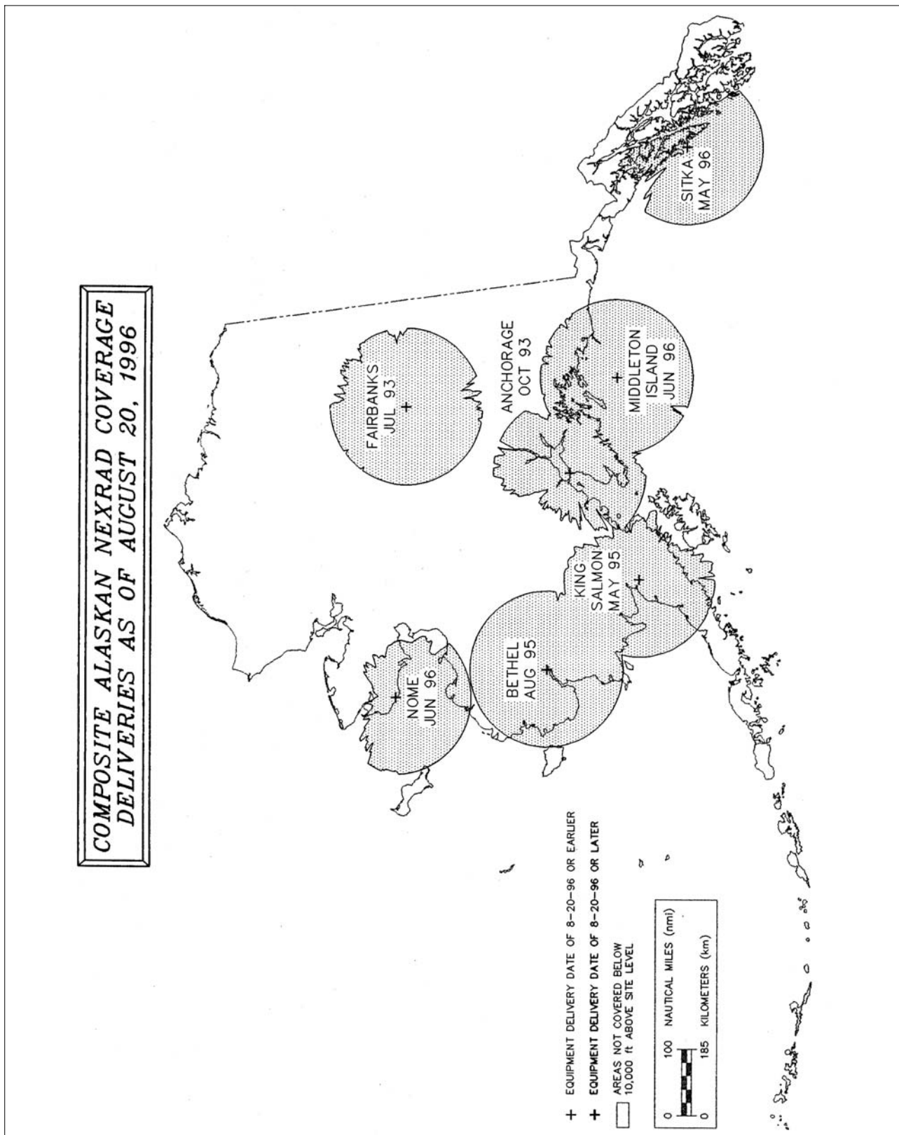
FIG 7-1-10 NEXRAD Coverage
