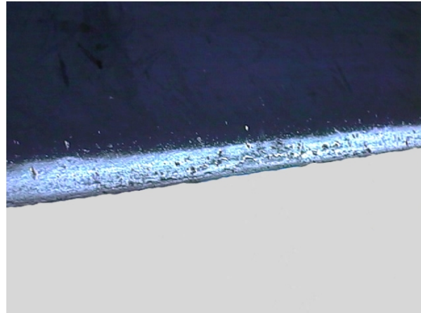
FIGURE 1-5. Exfoliation on the Blade Leading Edge
