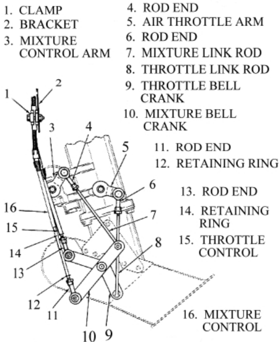
FIGURE 1. LINKAGE CONNECTION TO ENGINE
