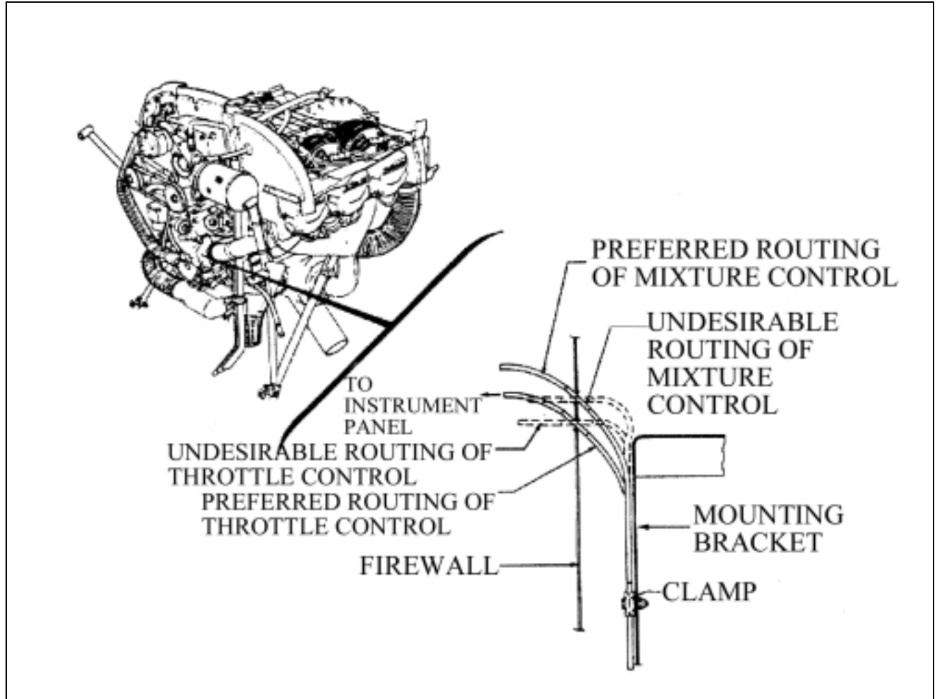
FIGURE 6. CONTROL CABLE BEND RADII
