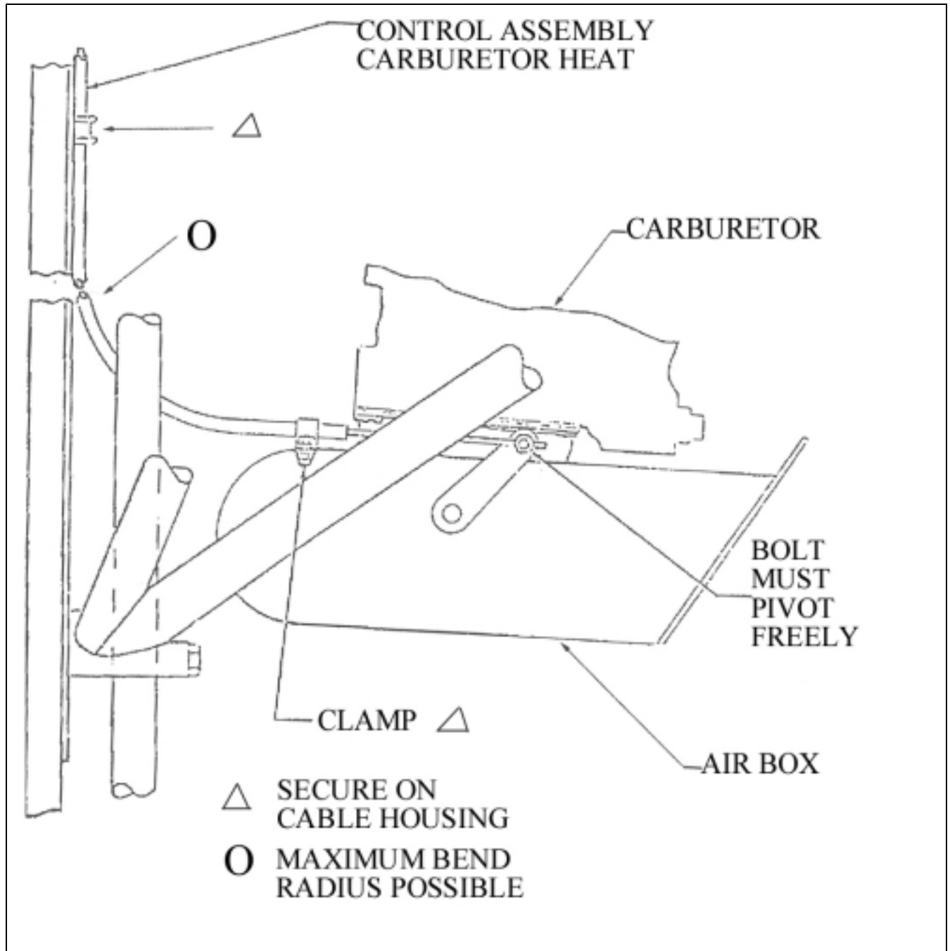
FIGURE 5. CONTROL ROUTING IN ENGINE COMPARTMENT
