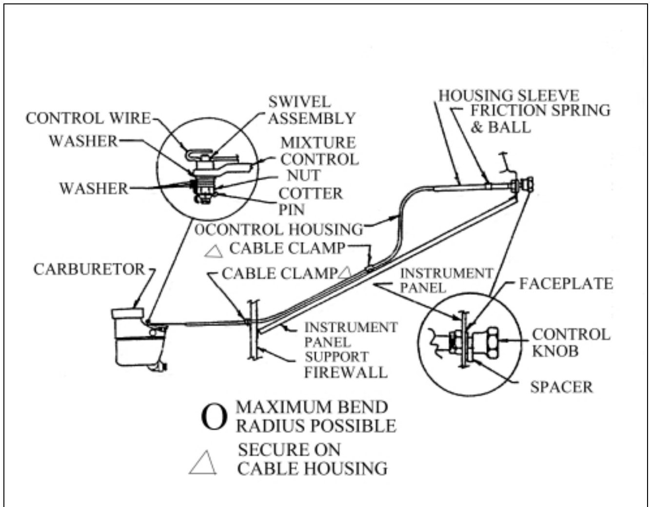
FIGURE 7. CONTROL SYSTEM OVERVIEW
