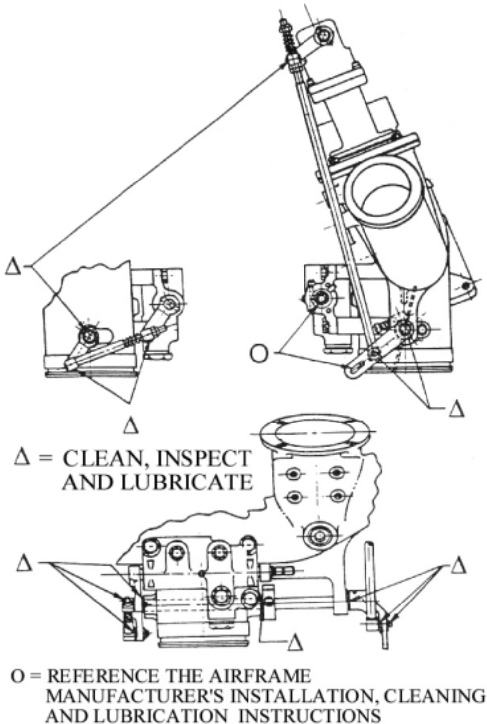
FIGURE 5. SOLID ROD ADJUSTMENT AND LUBRICATION
