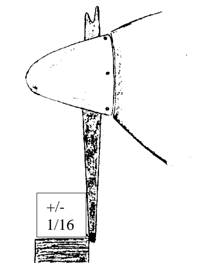
FIGURE 6. PROPELLER TRACKING
