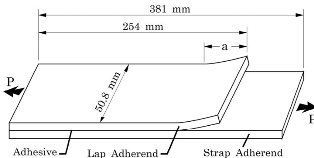
Figure 15.3-5 - Cracked lap shear (CLS) test specimen
