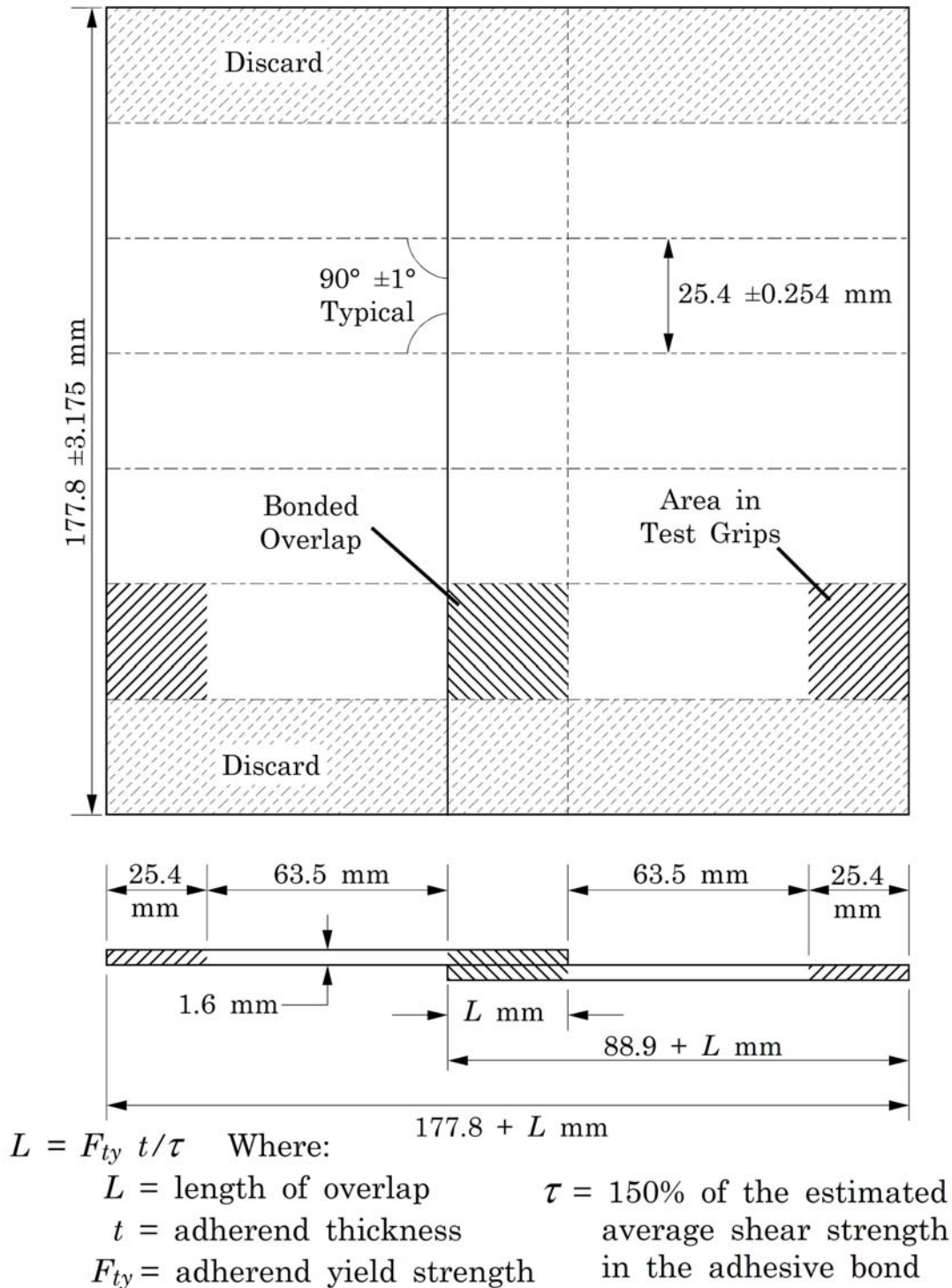
Figure 15.3-2 - ASTM D-1002: Single lap test specimen
