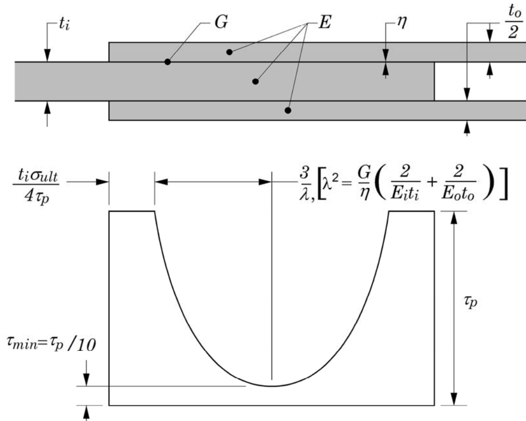
Figure 10.5-3 - Double lap joints: Design factors
