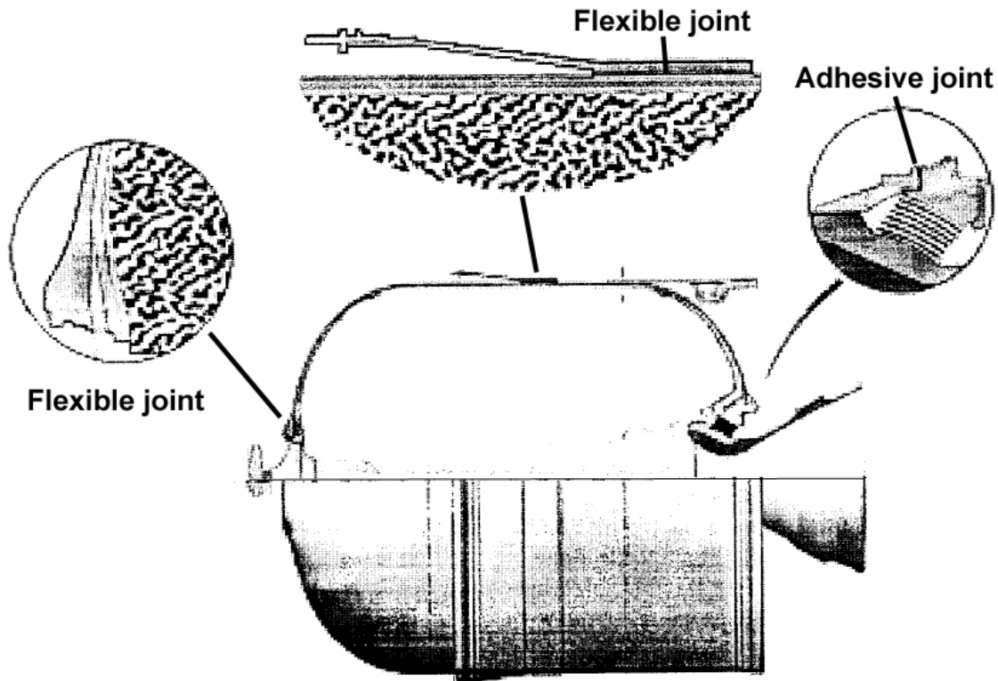
Figure 21.8-1 – Case study: SRM – position of flexible joints
