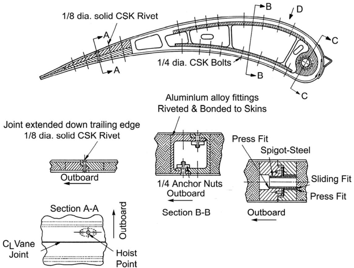
Figure 21.5-4 - Case study: MD 11 outboard flap vane - splice joint analysis
