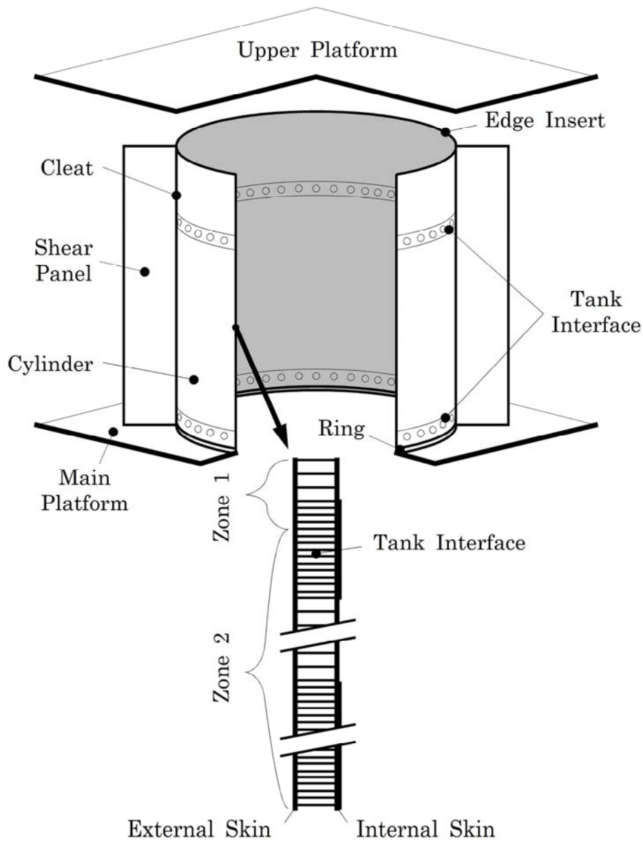
Figure 22.2-1 - Case study: CFRP central cylinder - structural elements
