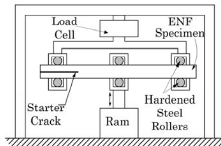
Fatigue loading fixture for End-notched Flexure Specimen
