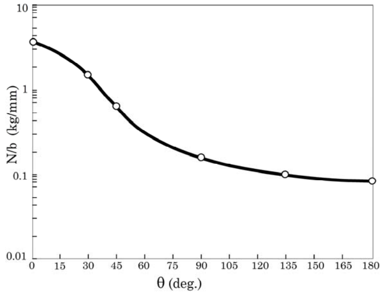
Figure 10.11-3 - \theta degree peeling strength
