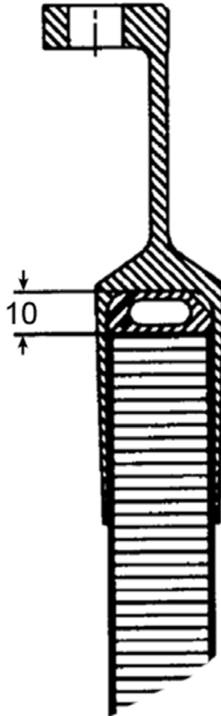
Figure 21.7-3 – Case study: Ariane 5 ACY 5400 - sectional view of bonded joint
