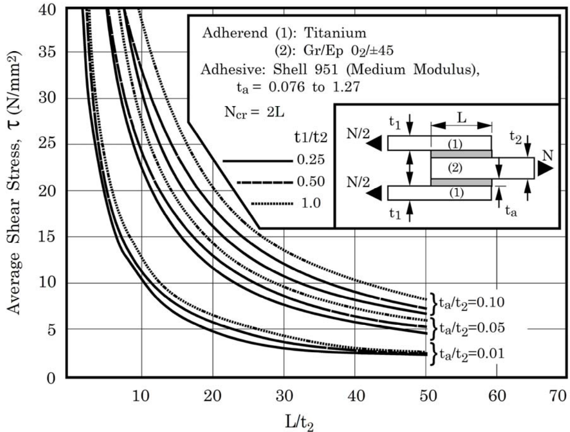
Figure 11.3-1 - Design curve: Static loaded double lap joint for CFRP/epoxy to titanium adherends
