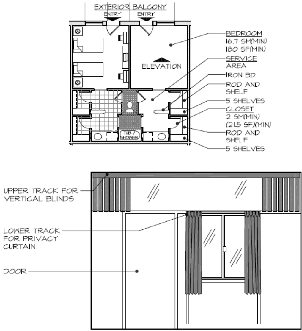
Figure B-9 Room Elevation
