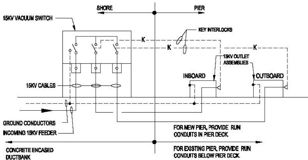
Figure E-5C Pier Electrical Distribution for Temporary Services (3 of 3)
