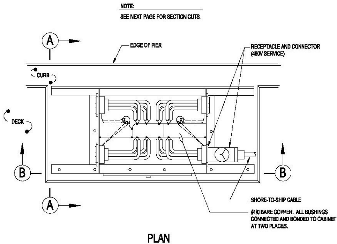
Figure E-4A Ship Service Outlet Assembly (1 of 2)
