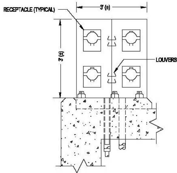
SECTION A
