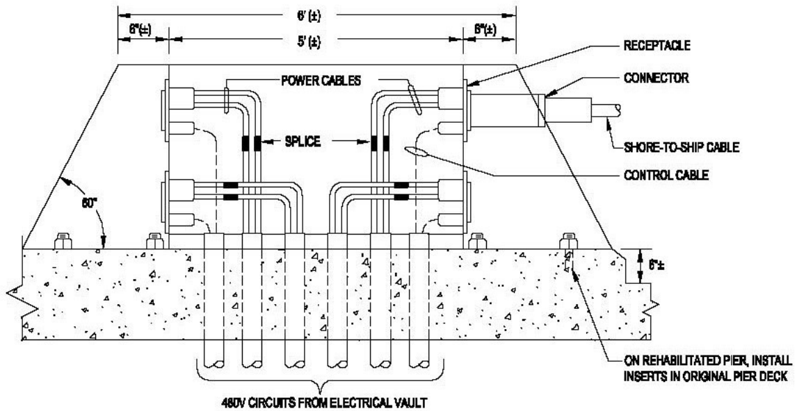
SECTION A
