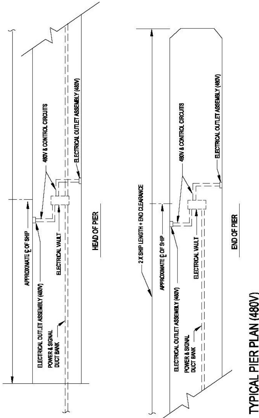
Figure E-2A Pier Electrical Distribution: Typical Vault System (1 of 5)
