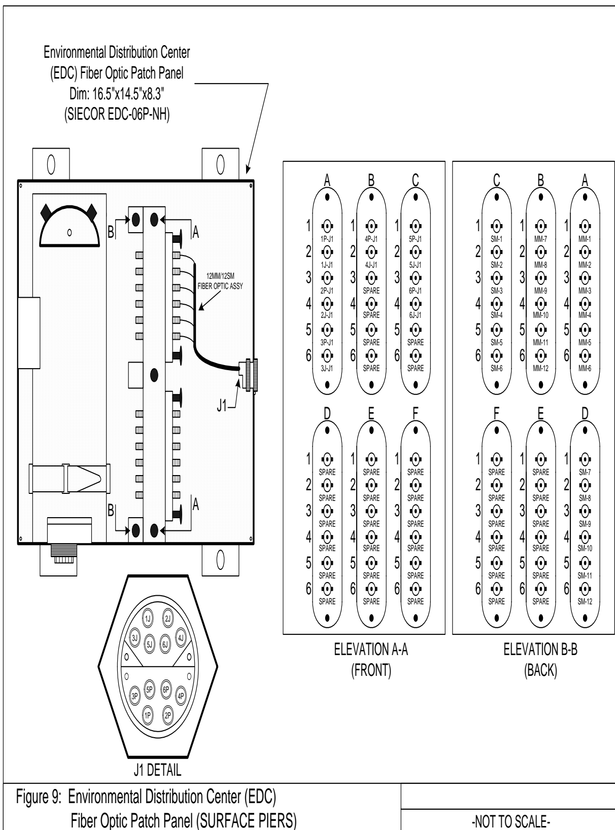
Figure 3-26 EDC Fiber Optic Patch Panel Surface Pier
