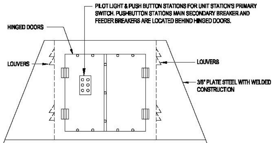
FRONT ELEVATION (REAR SIMILAR)
