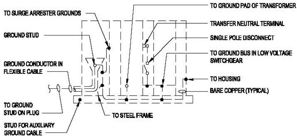
GROUNDING SCHEMATIC
