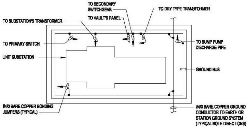
GROUNDING PLAN
