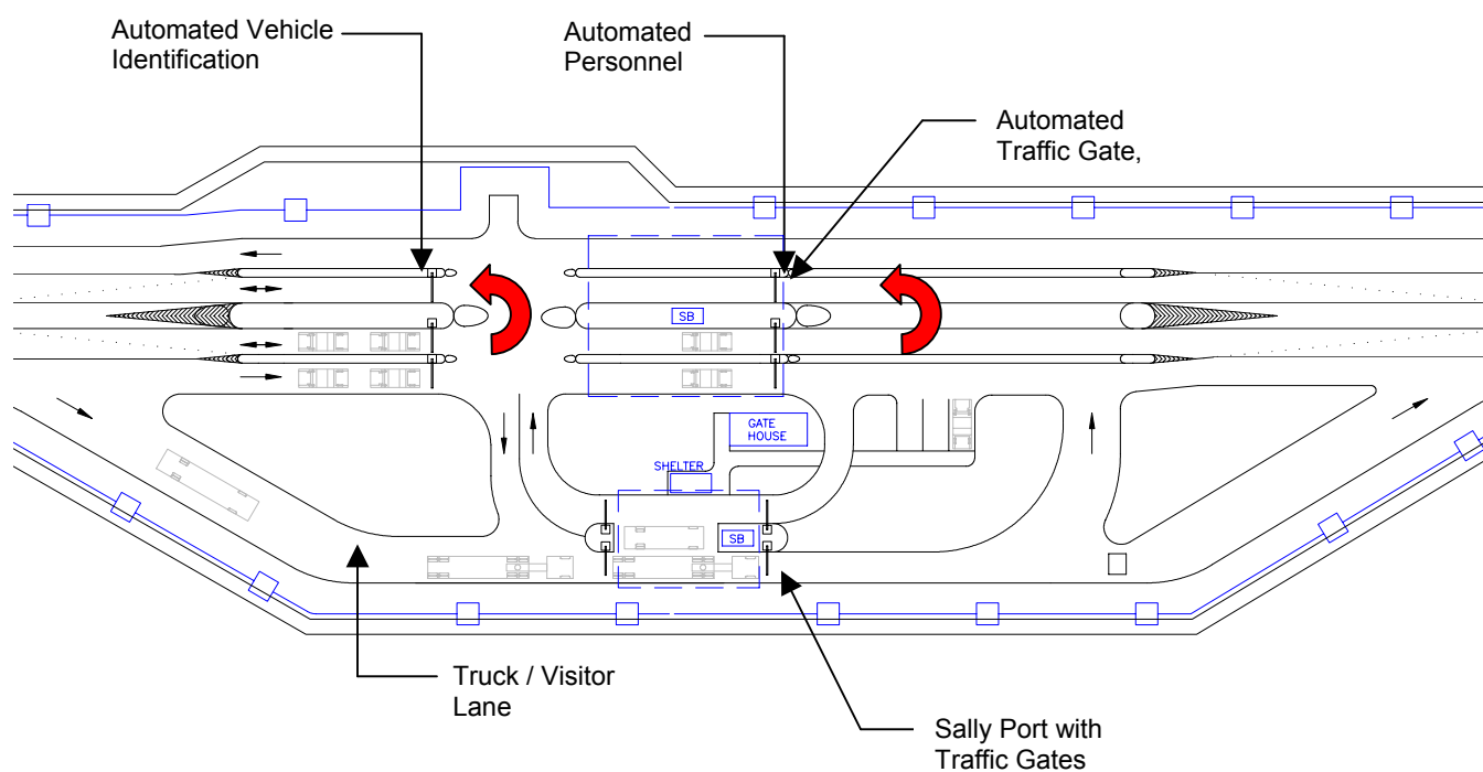
Figure 6-2 Access Control Zone Operated by Automated Equipment
