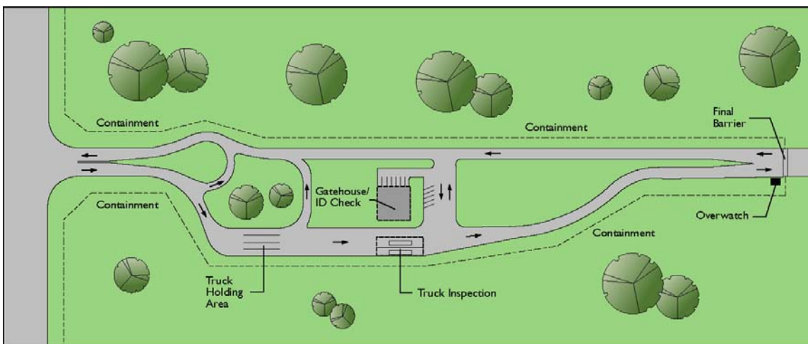
Figure 8-3 Commercial/Large Vehicle ECF
