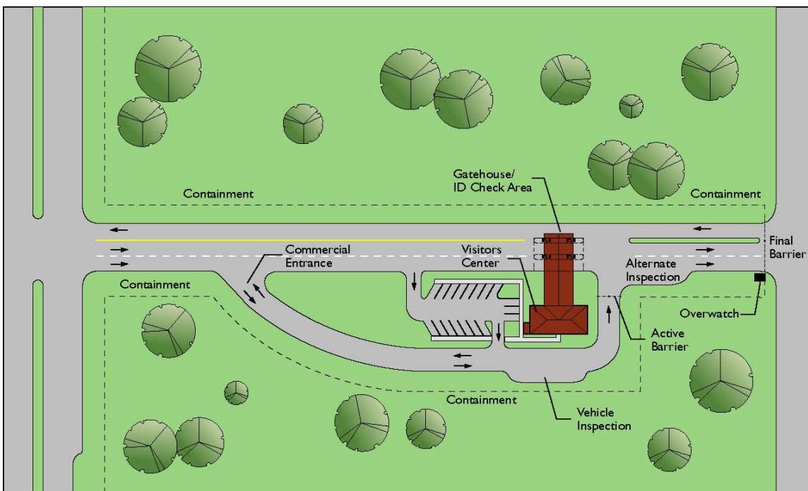
Figure 8-4 Combined Commercial/Visitors/DoD Alternative Gate
