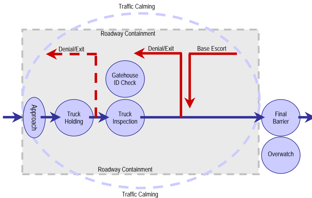
Figure 3-3 Commercial Gate: Functional Relationships
