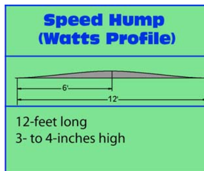
Figure 6-6 Example Speed Hump Profile
