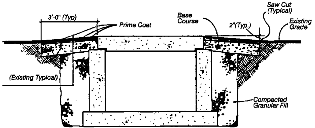
Parking Lot Pavement Cut Detail
