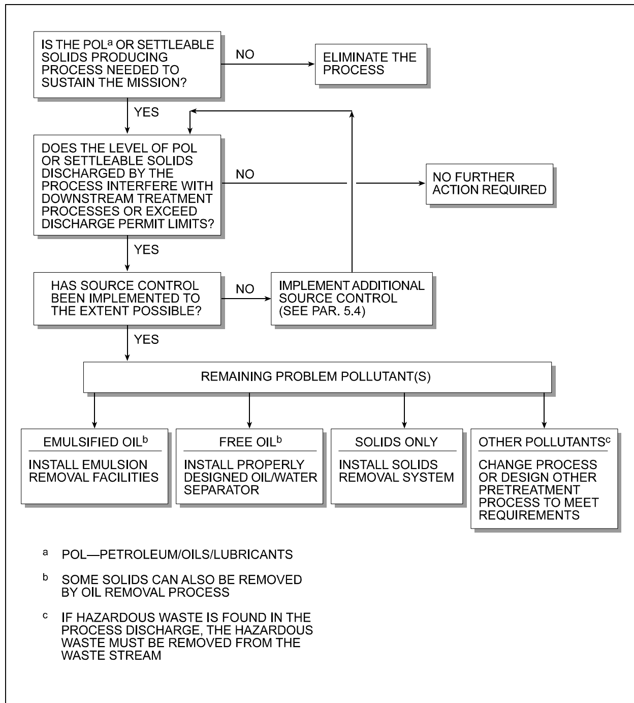
Figure 6 Decision Tree for Pretreatment of Oily Waste
