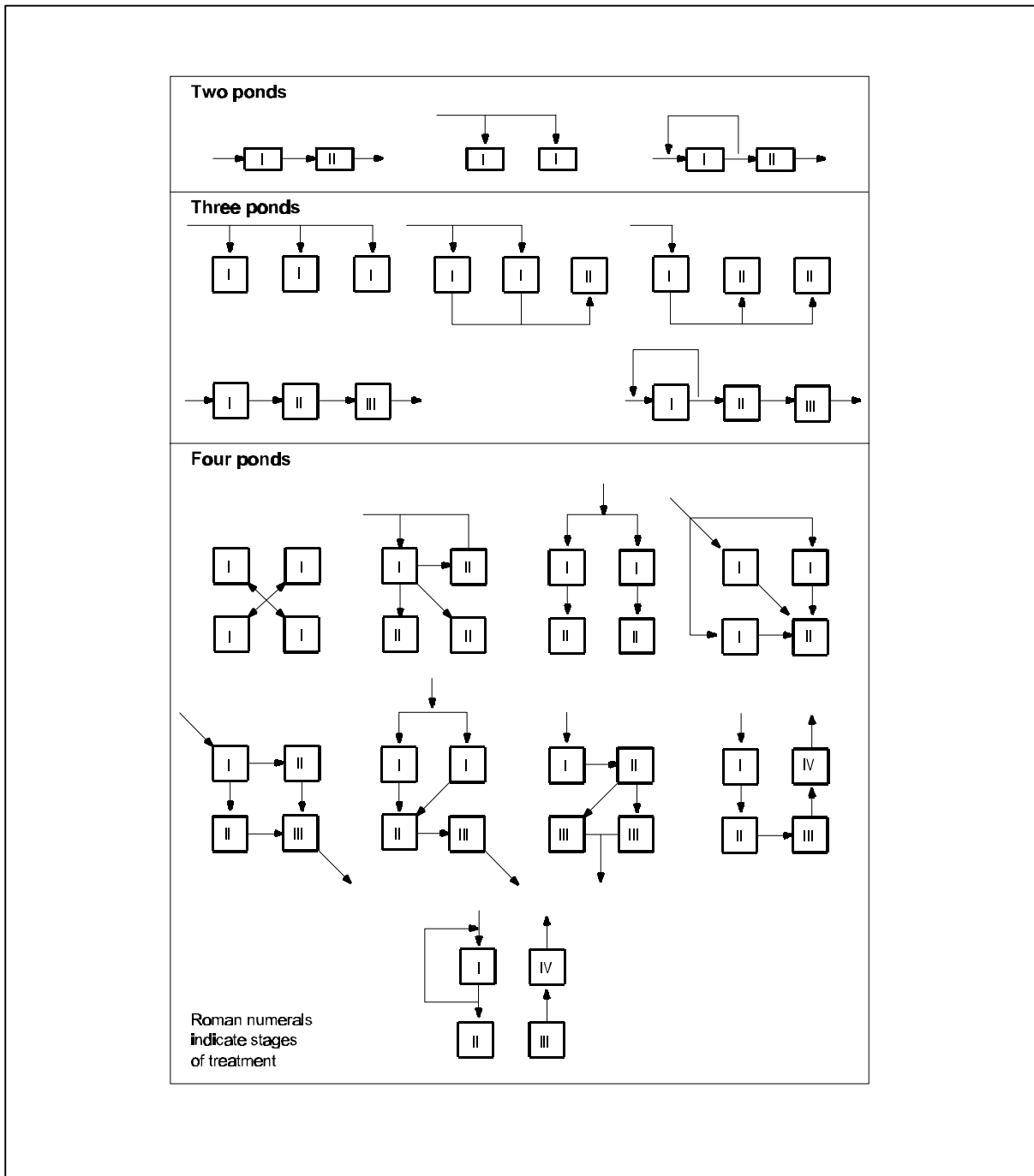
Figure 23 Alternative Lagoon Flow Schematics
