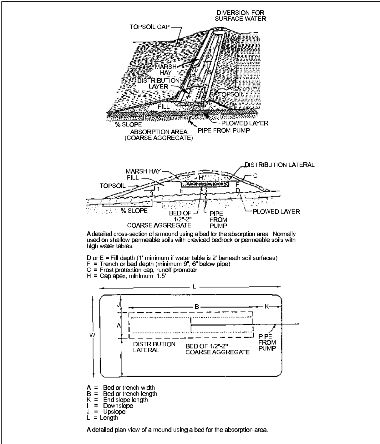
Figure 20 Mound System - Beds
