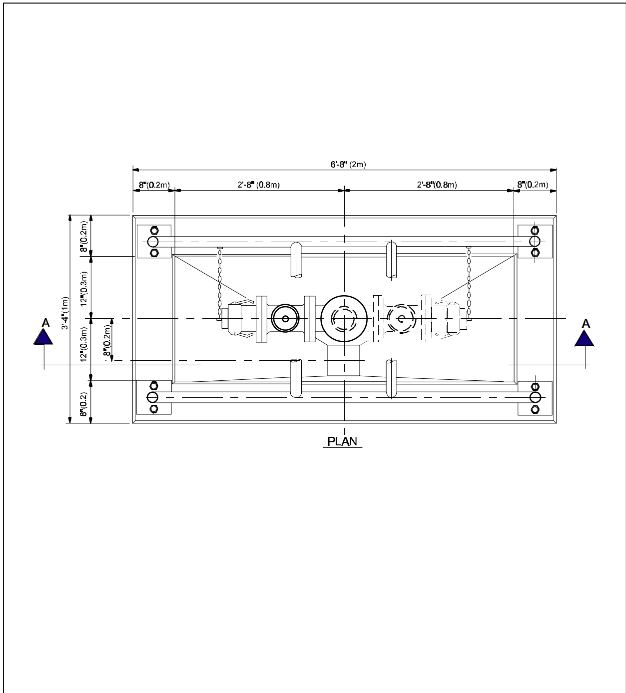
Figure 7 Aboveground Receiving Hose Connection
