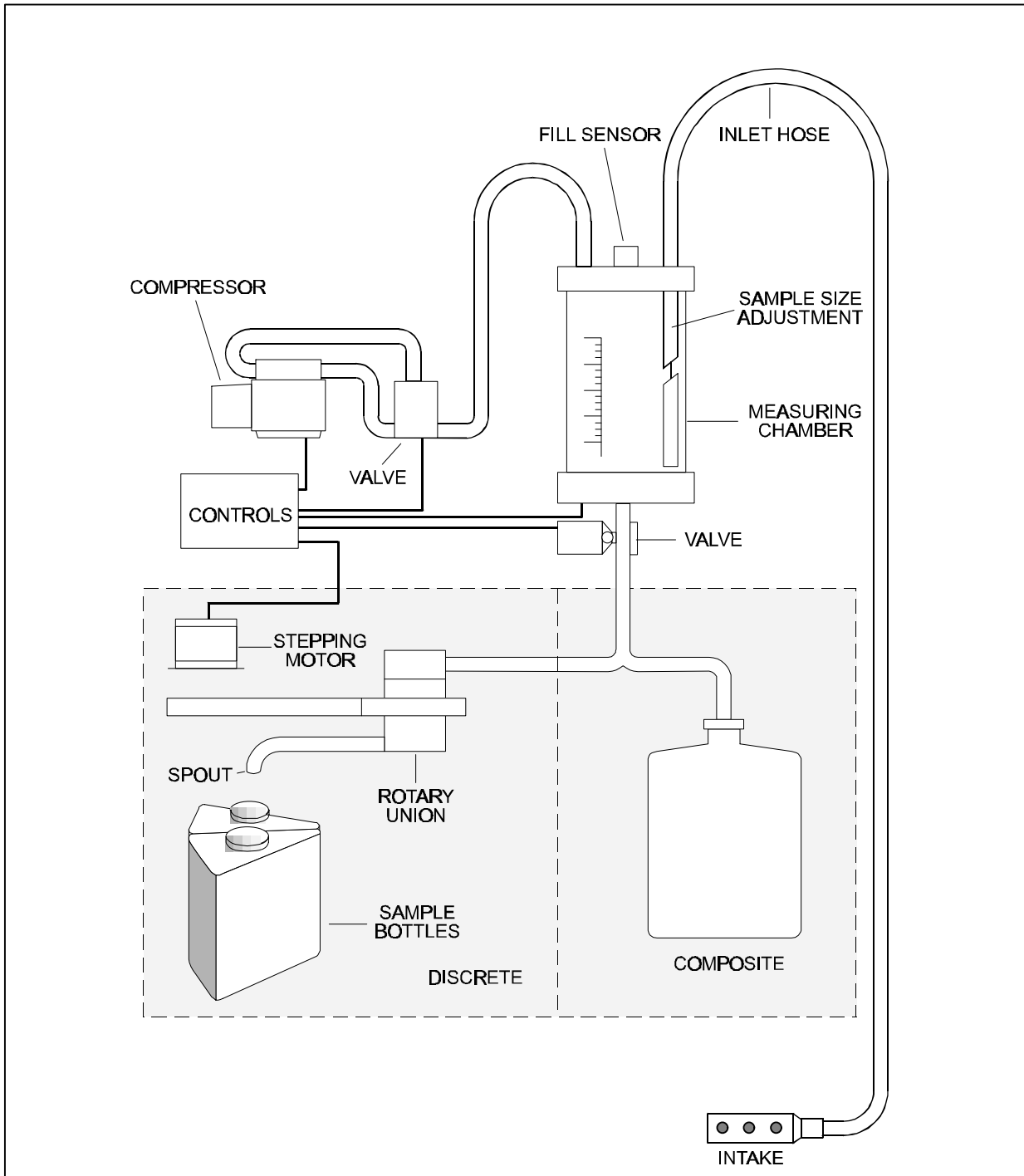
Figure 26 Schematic of Suction Lift Type Sampler
