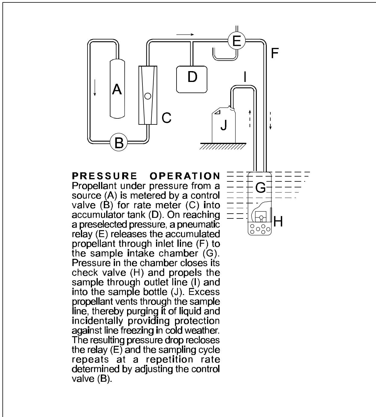
Figure 25 Schematic of Forced Flow Type Sampler
