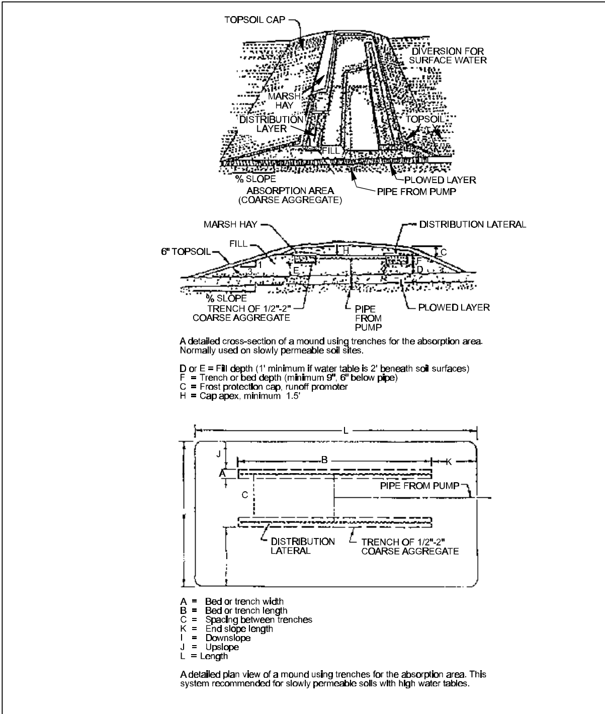
Figure 19 Mound System - Trenches
