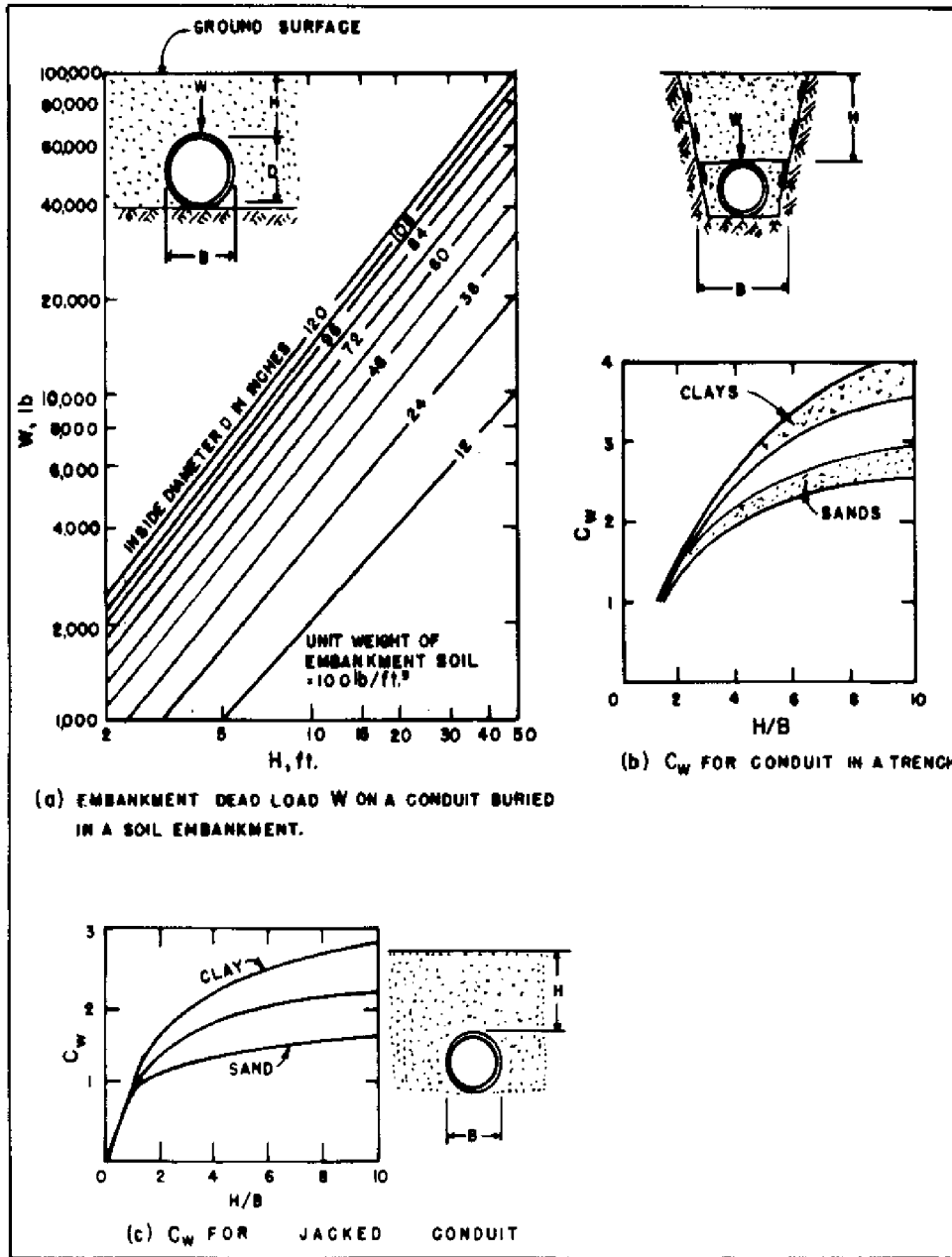
FIGURE 18 Backfill Coefficients, Embankment Loads, and Load Factors for Rigid Conduits
