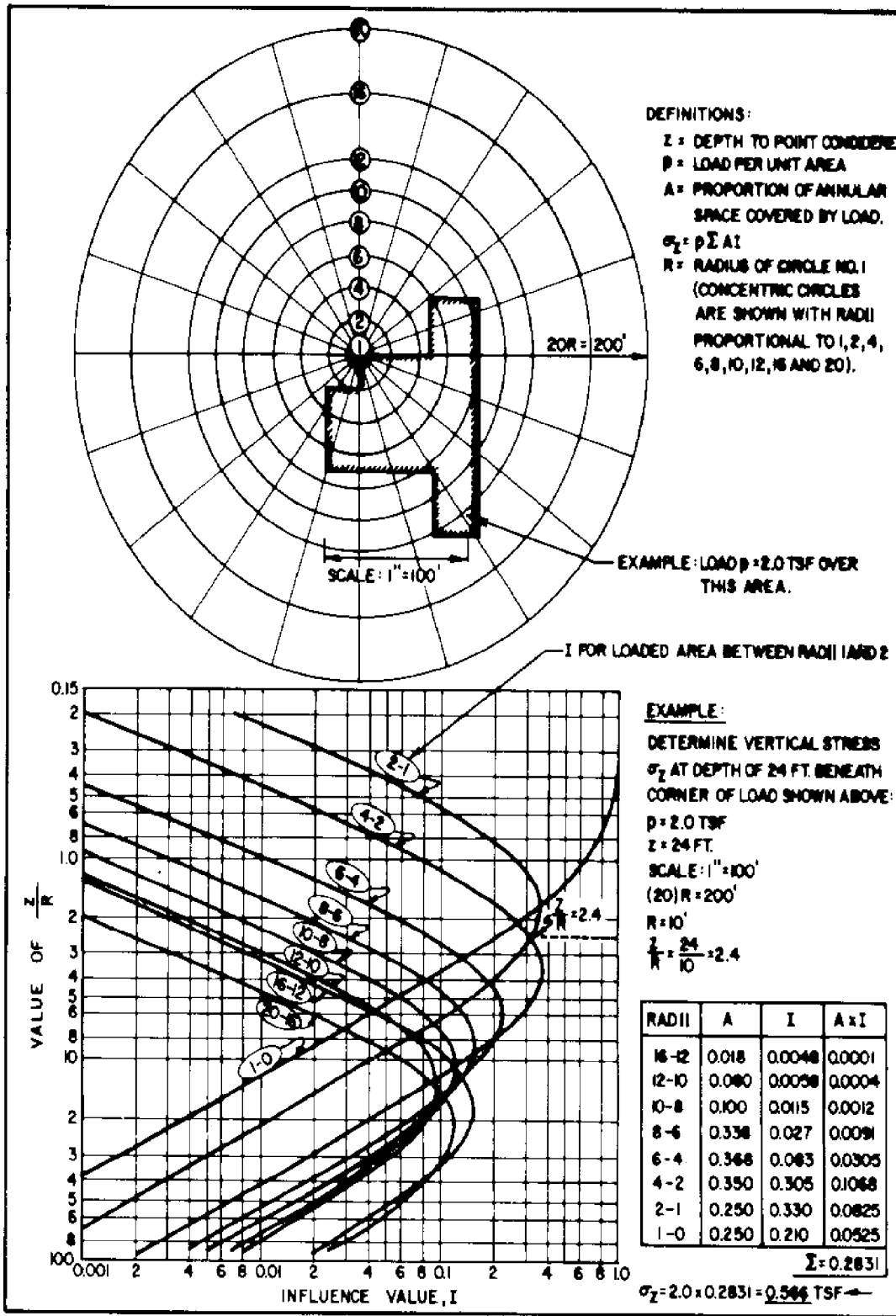
FIGURE 10 Influence Chart for Vertical Stress Beneath Irregular Load
