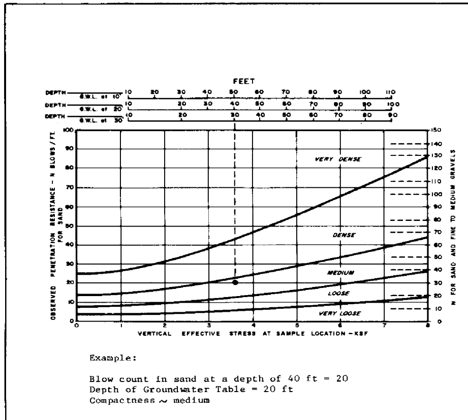
FIGURE 1 Estimated Compactness of Sand from Standard Penetration Test
