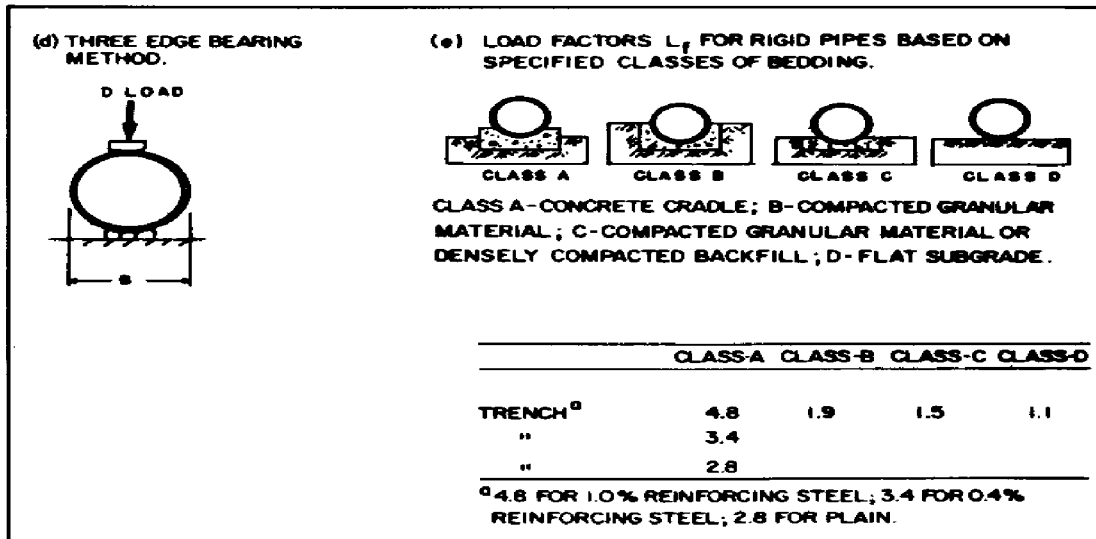
FIGURE 18 (continued) Backfill Coefficients, Embankment Loads, and Load Factors for Rigid Conduits
