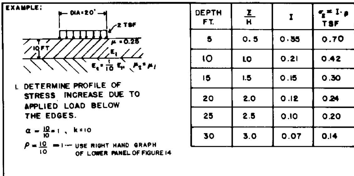
FIGURE 15 Stress Profile in a Two-Layer Soil Mass
