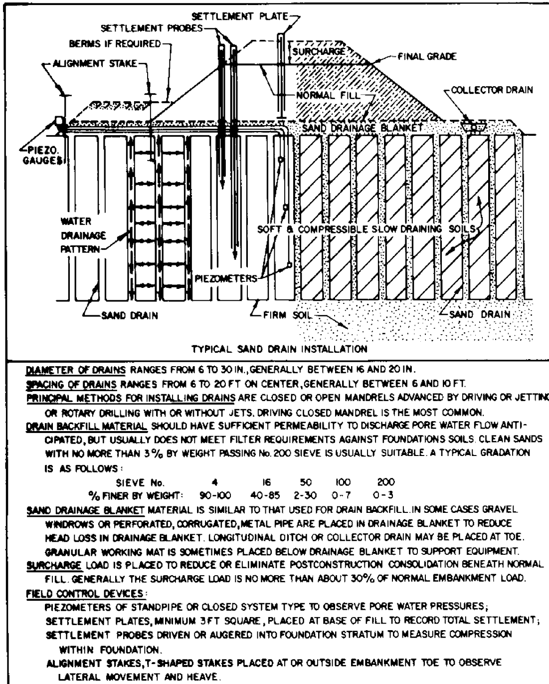
FIGURE 18 Data for Typical Sand Drain Installation
