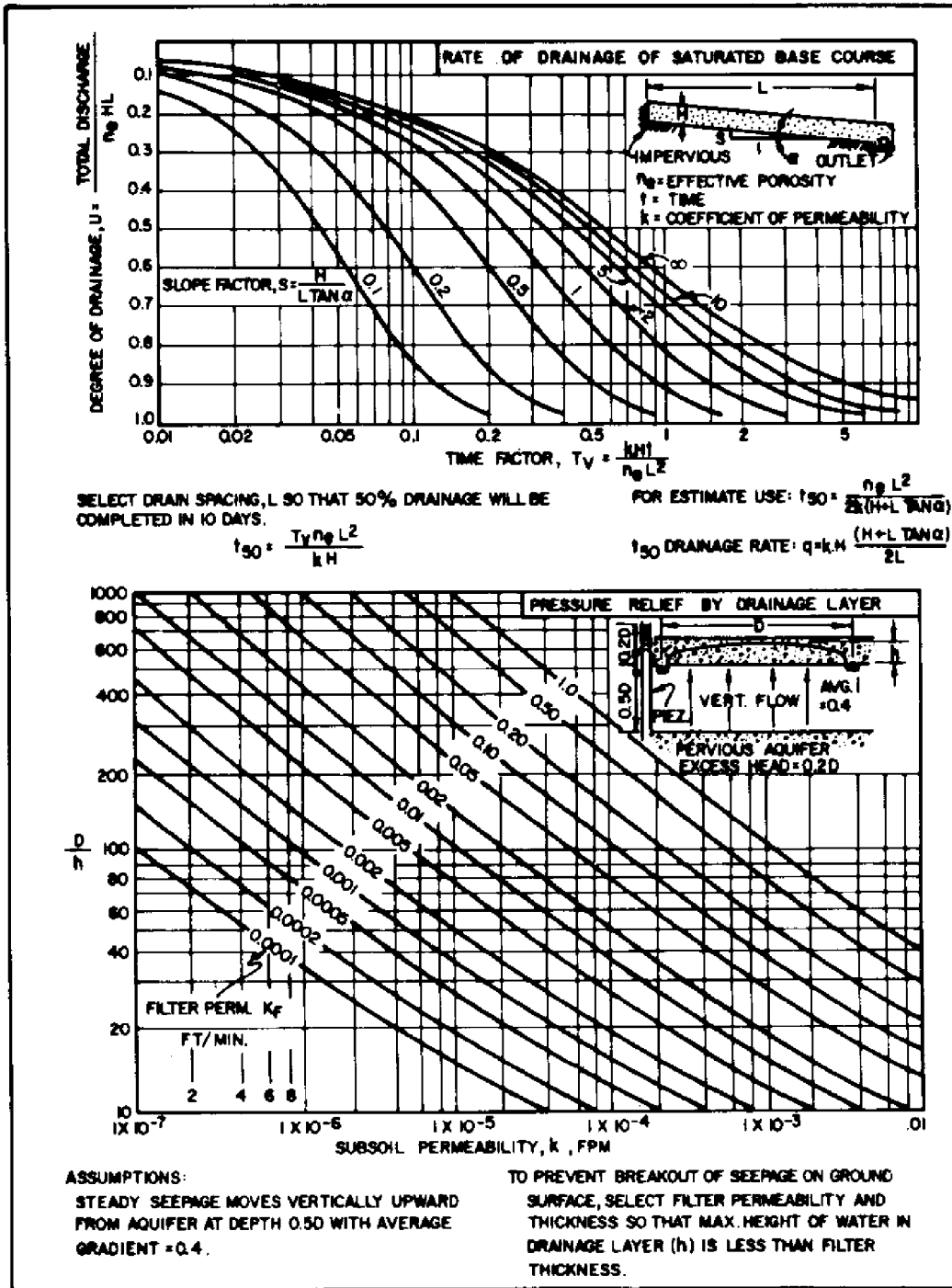
FIGURE 7 Analysis of Drainage Layer Performance
