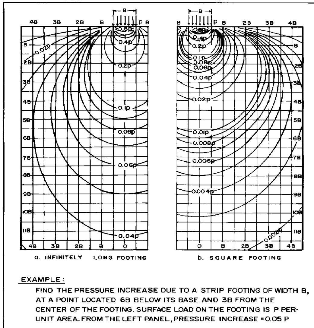
FIGURE 11 Vertical Stress Contours for Square and Strip Footings (Westergaard Case)
