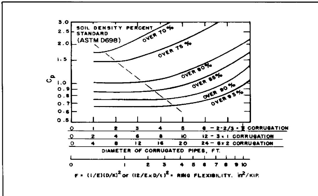
FIGURE 20 Pressure Transfer Coefficients for Corrugated Flexible Conduits as a Function of Standard Soil Density and Ring Flexibility or Diameter and Corrugation Depth
