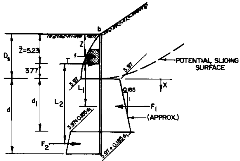
FIGURE 13 Example Calculation - Pile Stabilized Slopes
