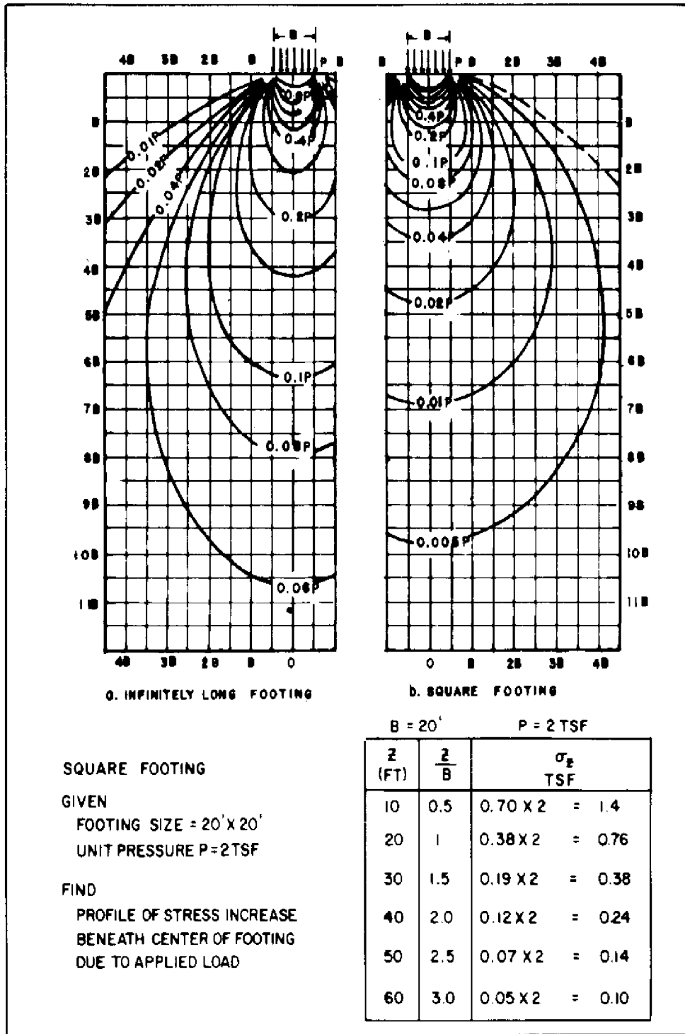
FIGURE 3 Stress Contours and Their Application
