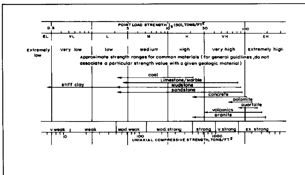
FIGURE 3 Strength Classification
