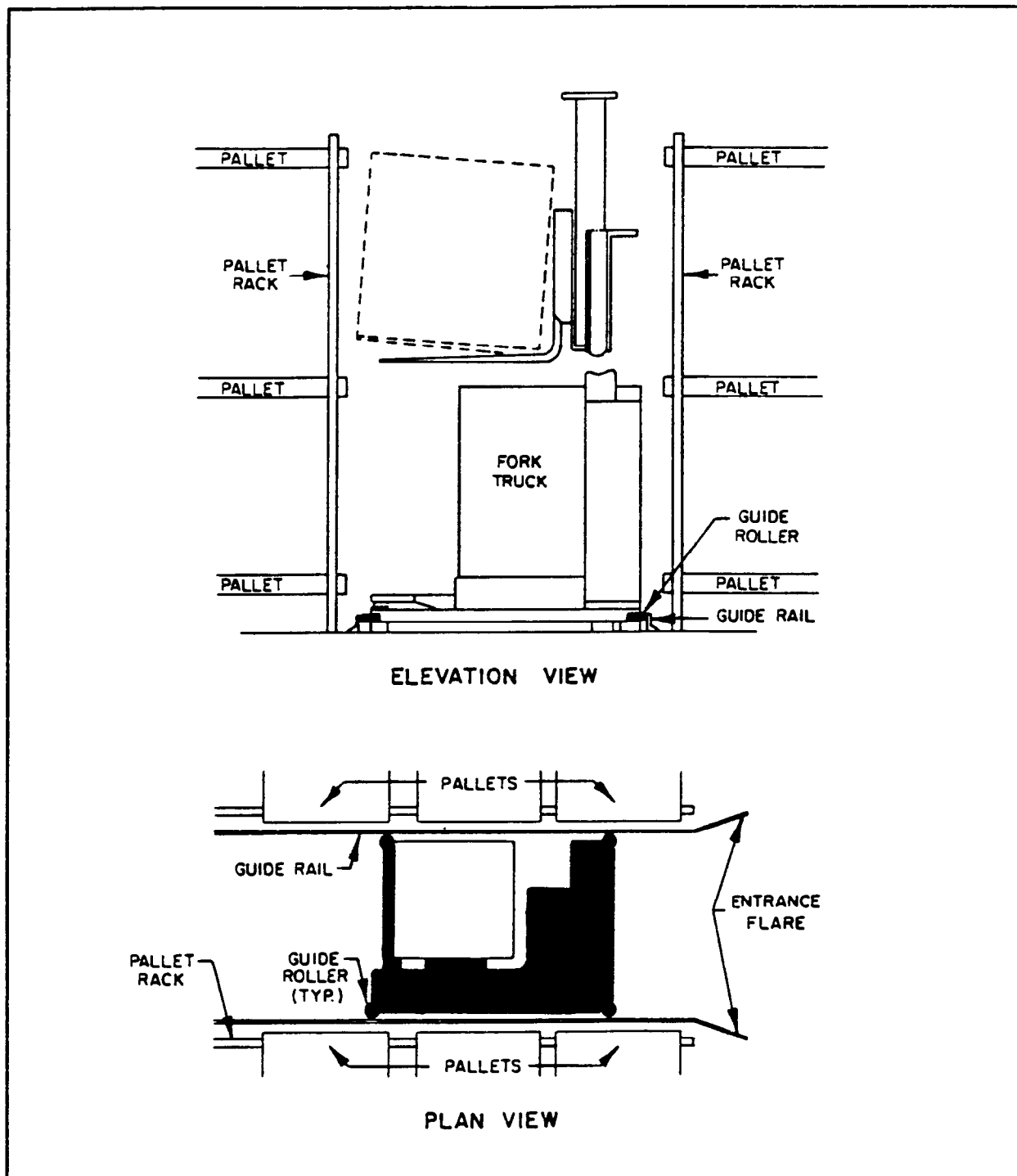
Figure 30 Typical Rail Guidance System
