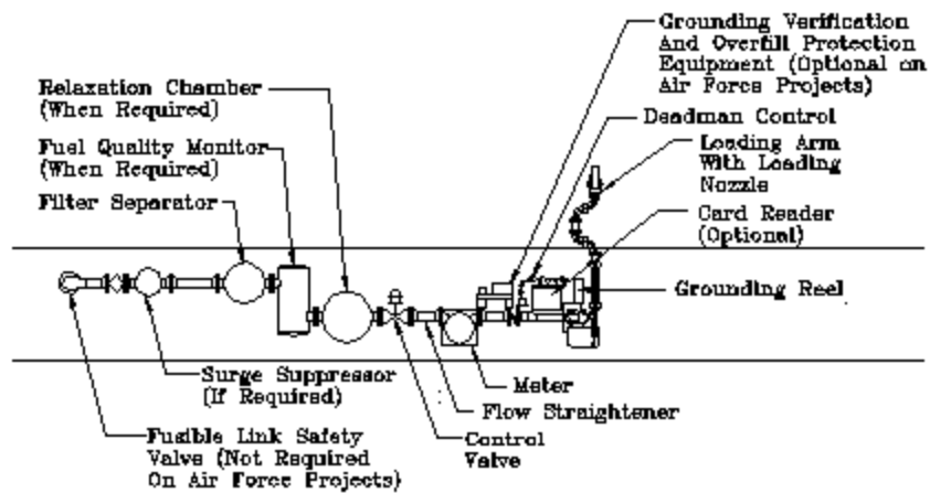
LOADING EQUIPMENT - STAND ALONE
