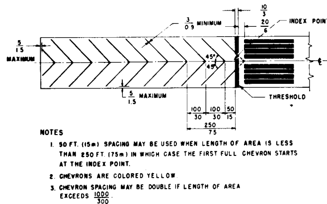
(b) MARKINGS FOR BLAST PADS AND STOPWAYS
