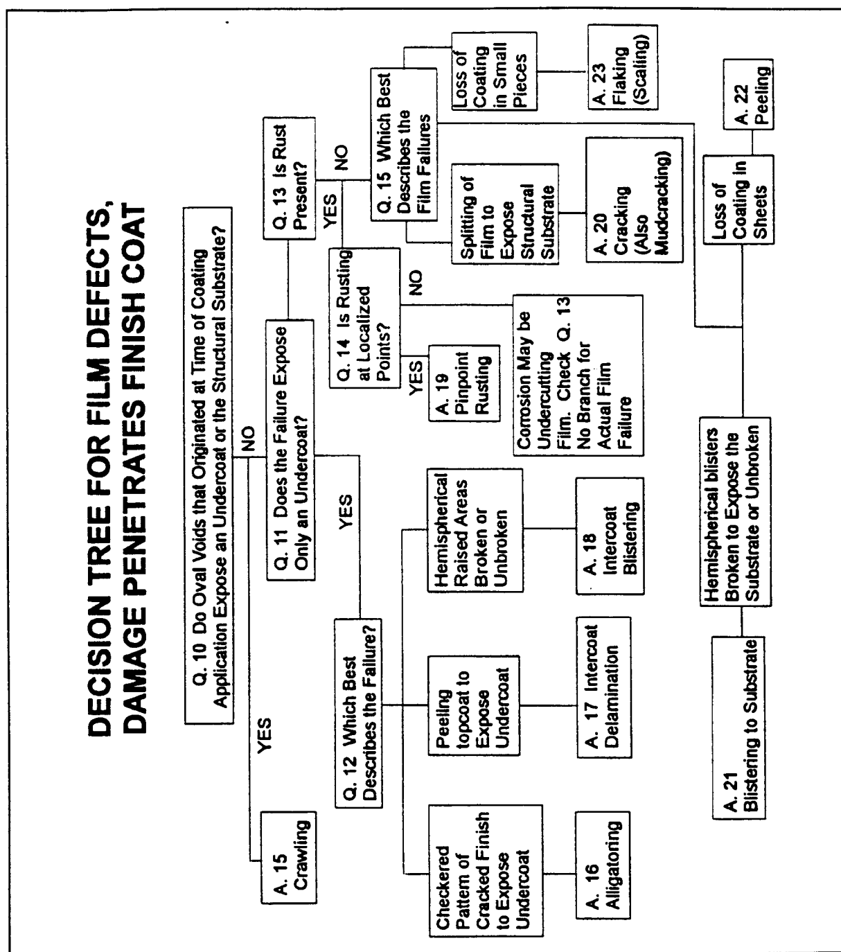
Figure 25 Decision Tree 2: Support for Analysis of Coating Defects That Penetrate the Finish Coat
