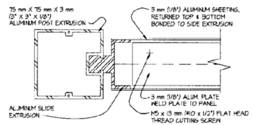
S4 ALT. HORIZONTAL SECTION (EXTRUDED POST)
