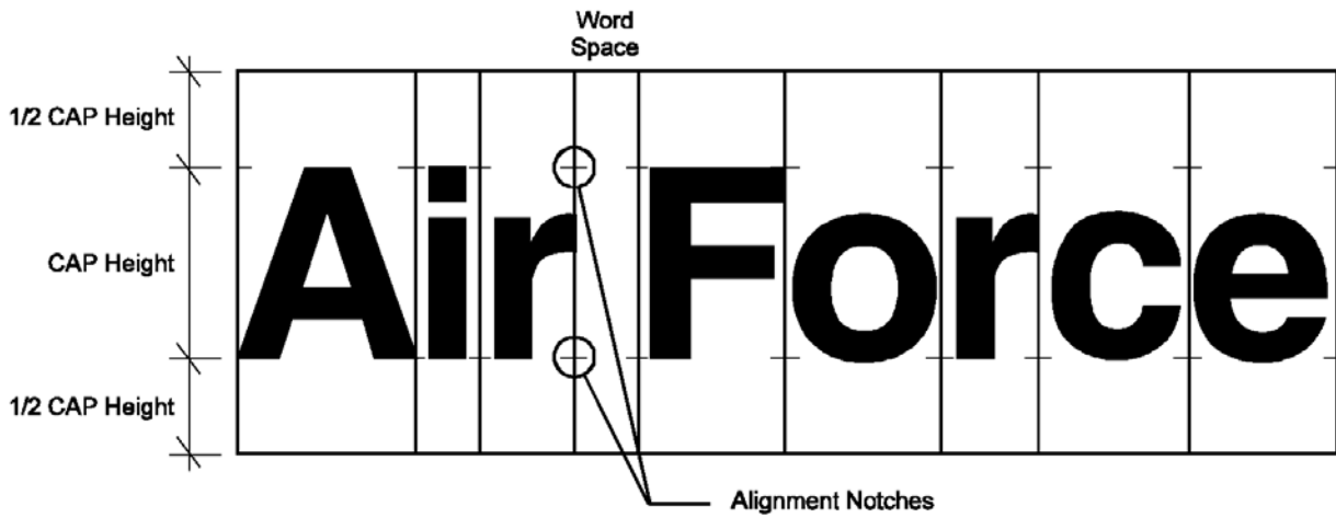
Figure 2.7. Sign Grid.
