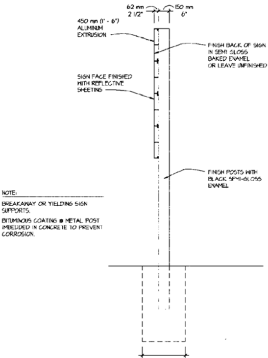
SECTION SCALE 1/4"=1'-0"
