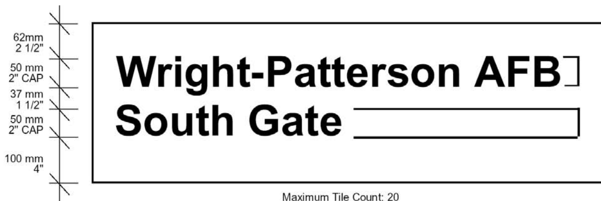
Figure 4.10. Entry Gate Type A3 Expanded Layout.
