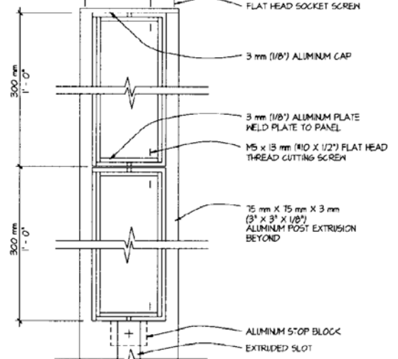
S5 ALTERNATE VERTICAL SECTION
