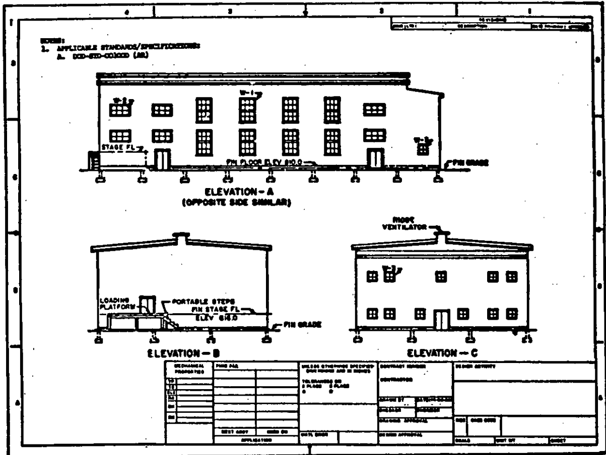
FIGURE 200-20. Elevation drawing
