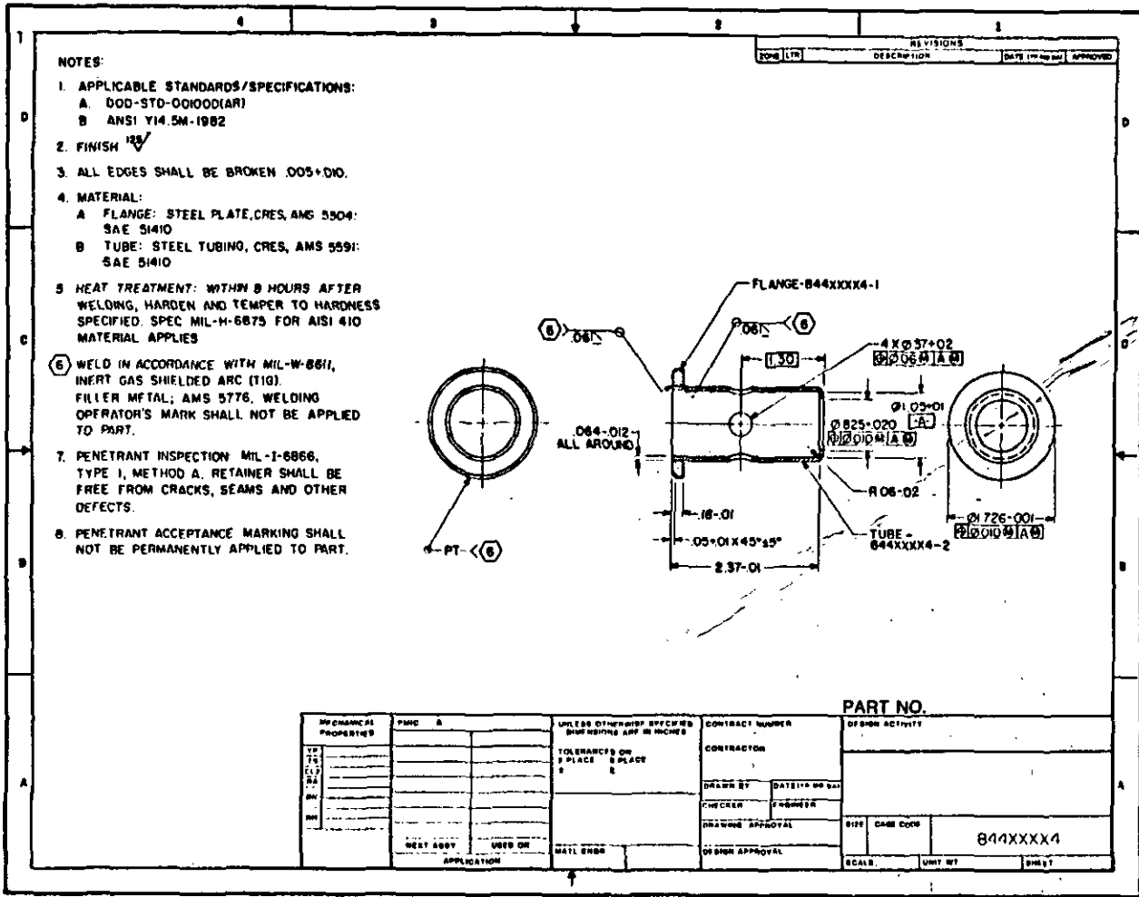
FIGURE 200-9. Inseparable assembly drawing
