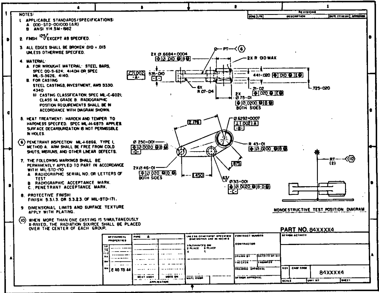
FIGURE 200-1. Monodetail drawing
