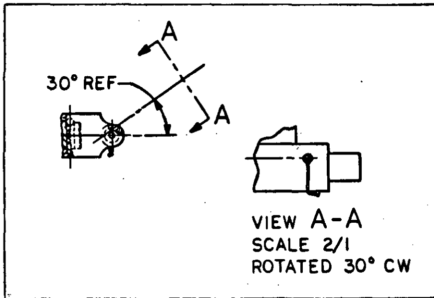
FIGURE 100-2. Auxiliary and Sectional View Rotation From Perpendicular Projection
