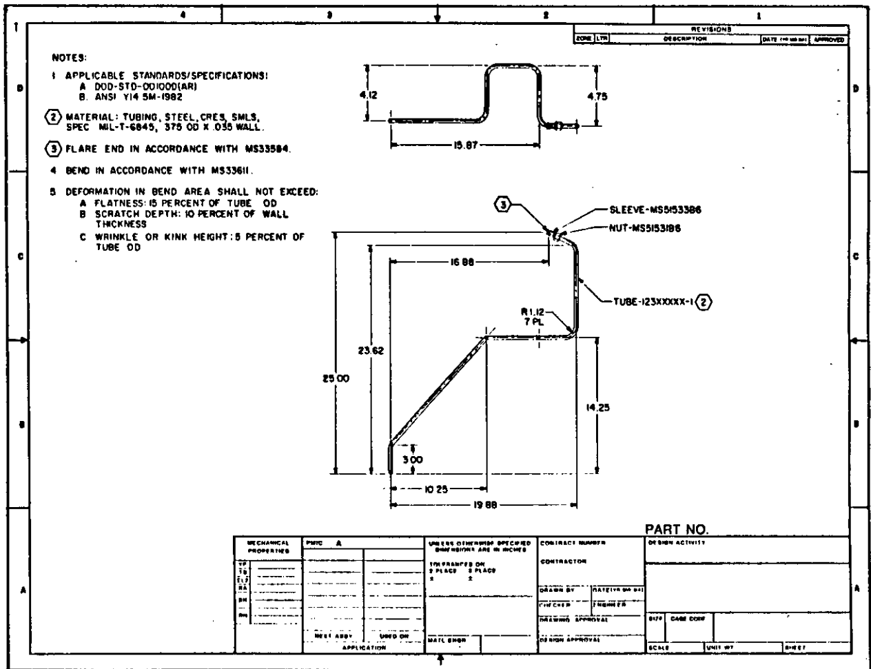
FIGURE 200-4. Tube bend drawing
