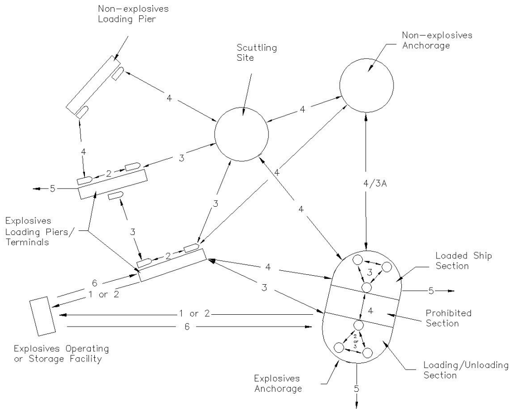
Figure C9.F10. Application of Separation Distances for Ship or Barge
