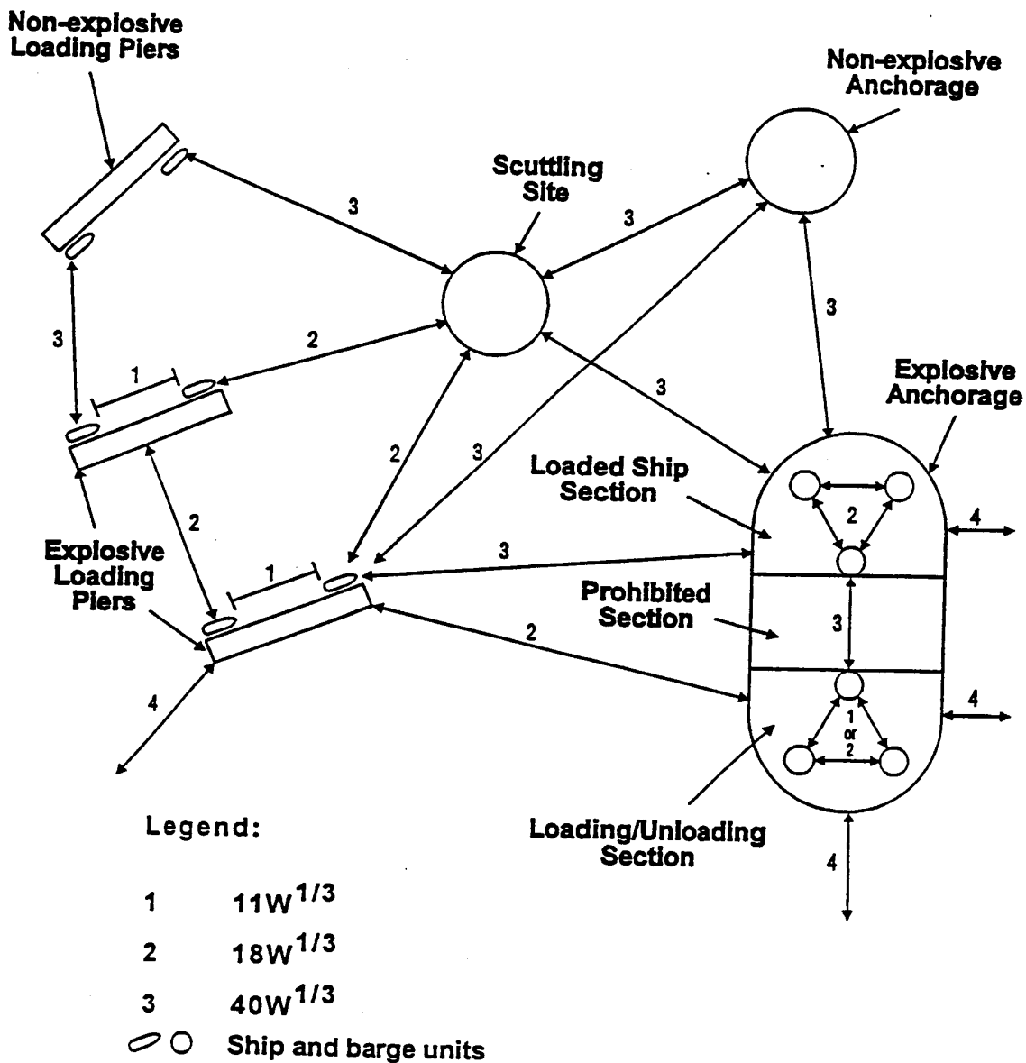
Figure C6.F2. Application of Separation Distances for Ship and Barge Units.
