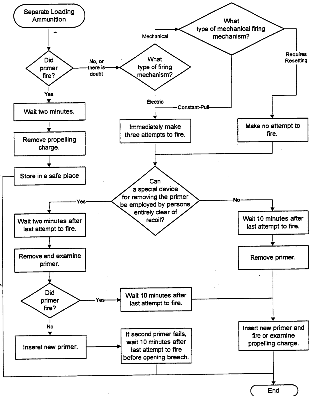
Figure C14.F8. Misfire of Separate Loading Ammunition.
