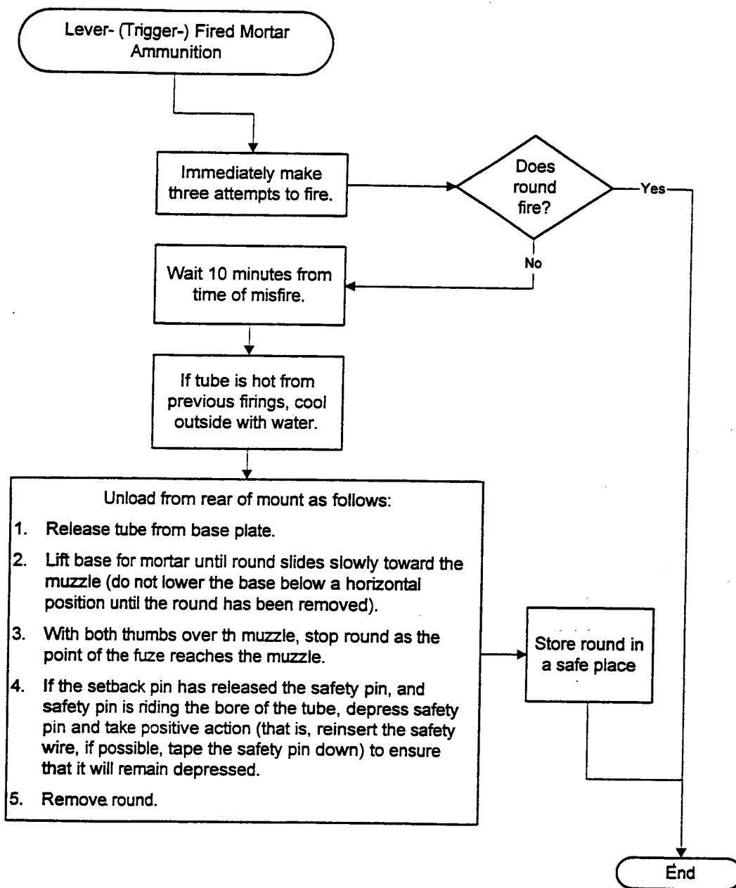
Figure C14.F5. Misfire of Lever- (Trigger-) Fired Mortar Ammunition.
