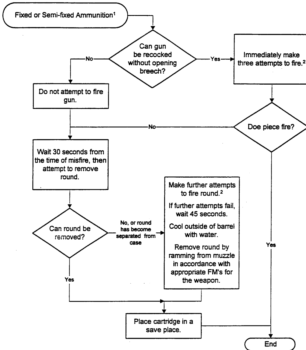
Figure C14.F3. Misfire of Fixed or Semi-fixed Ammunition.
