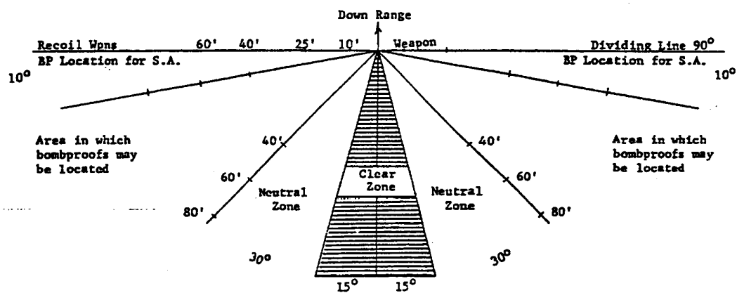
Figure C14.F9. Emplacement of Bombproofs at Firing Points.
