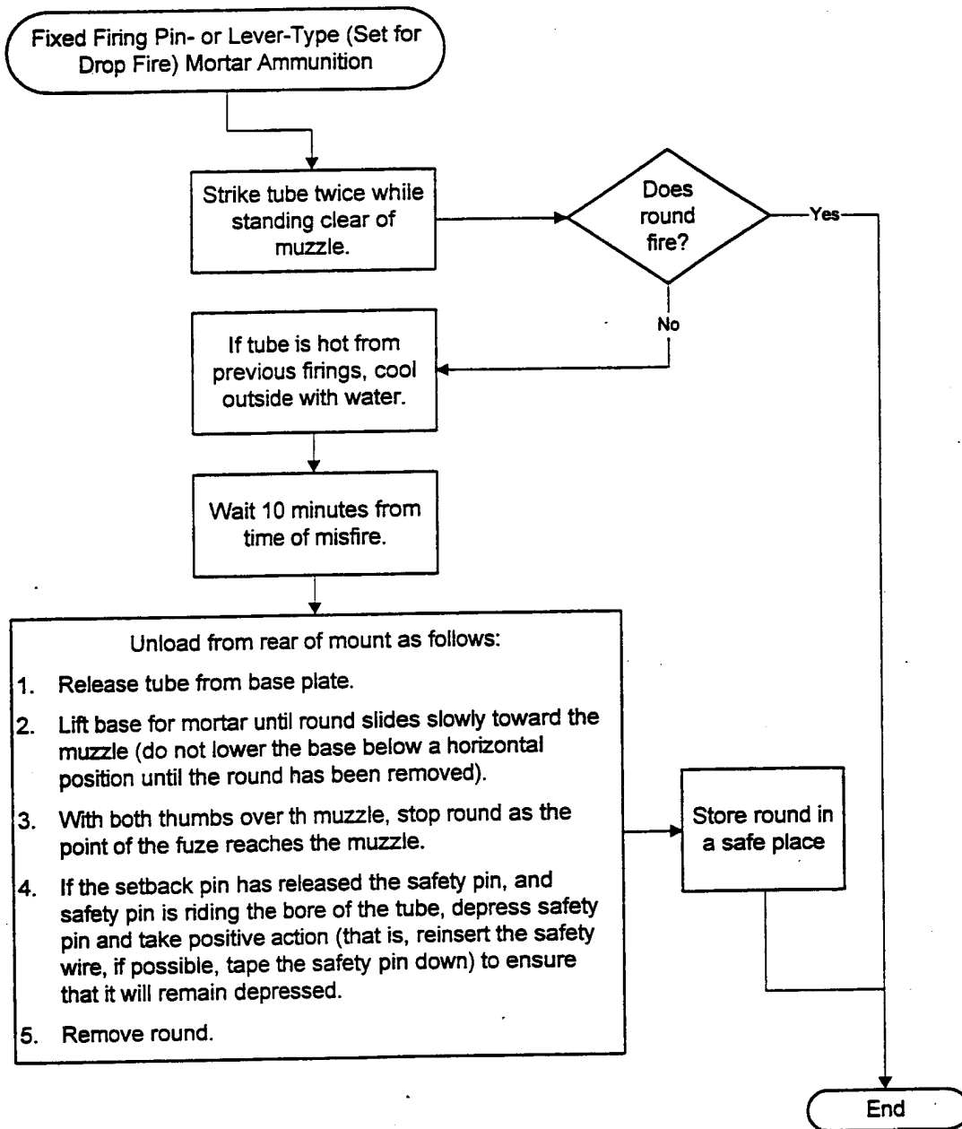
Figure C14.F6. Misfire of Fixed Firing Pin- or Lever-Type (Set for Drop Fire) Mortar Ammunition.
