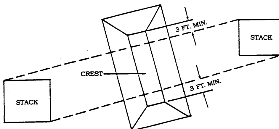
Figure C4.F3. Determination of Barricade Length.
