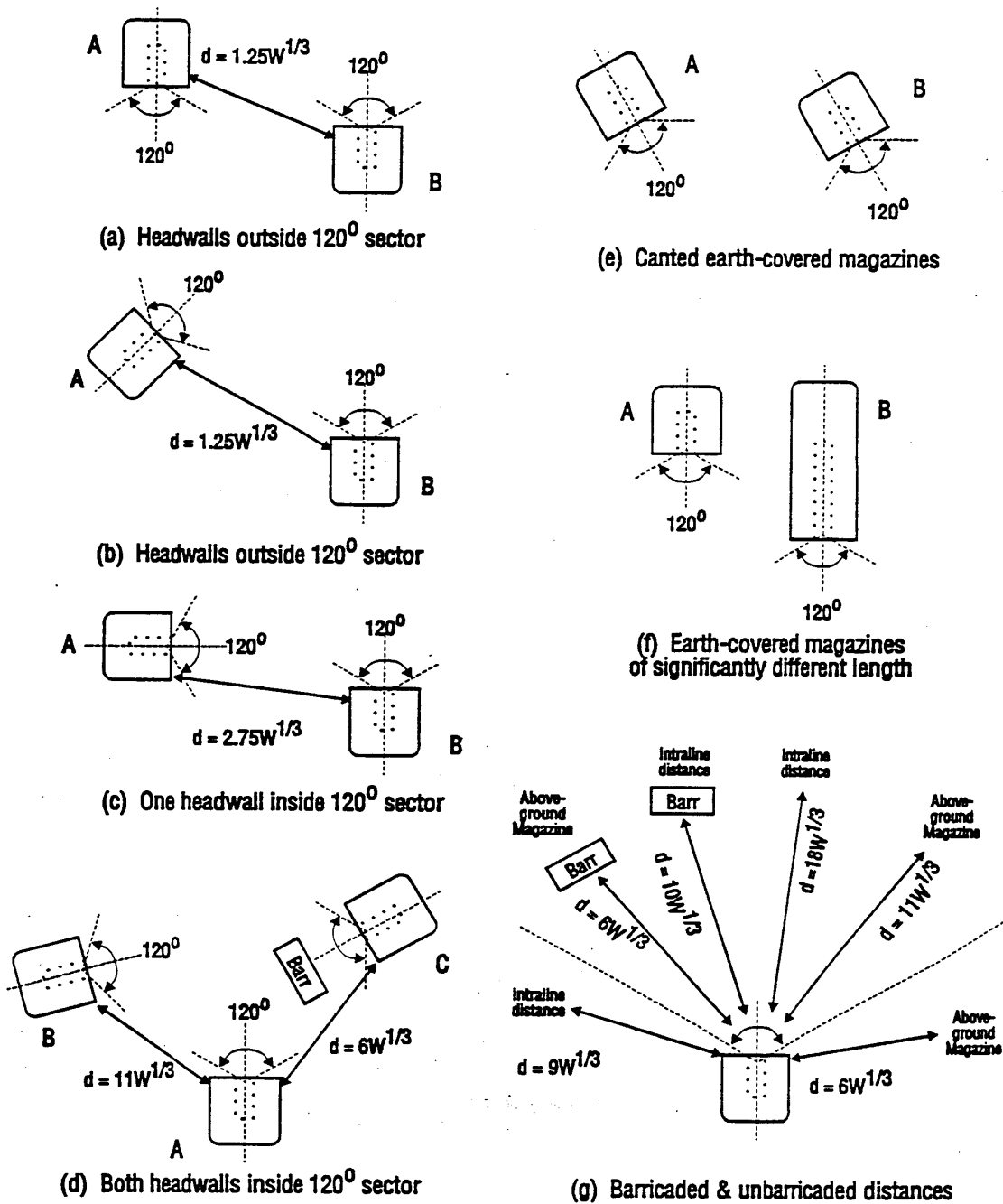
Figure C6.F1. Effects of Magazine Orientation on Q-D.
