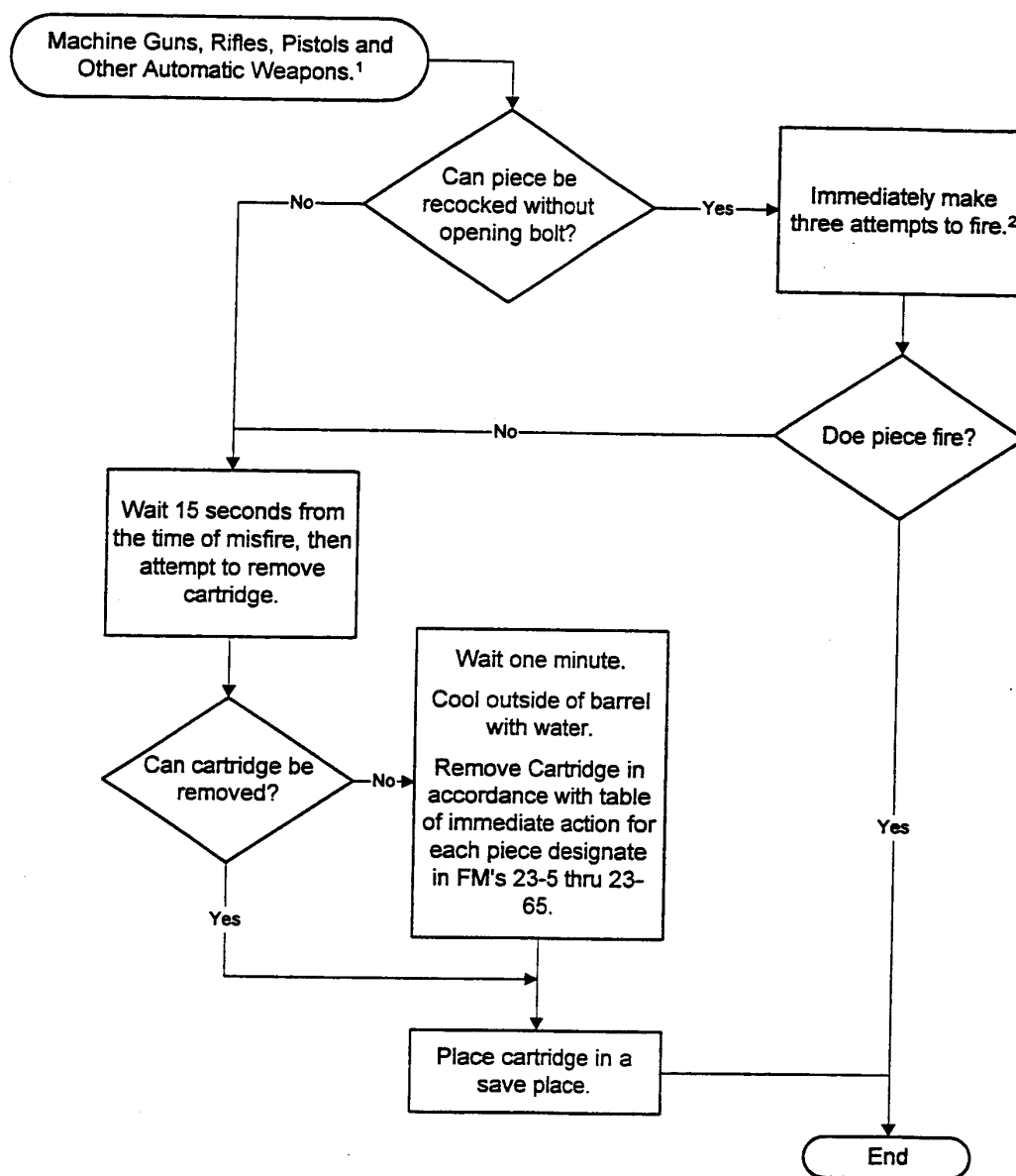
Figure C14.F1. Misfire of Machine Guns, Rifles, Pistols, and Other Automatic Weapons.
