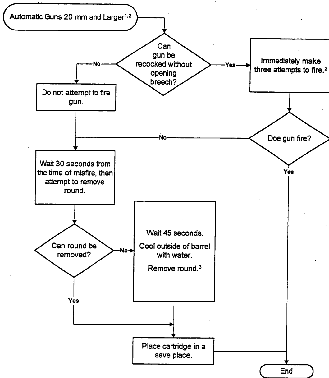
Figure C14.F2. Misfire of Automatic Guns, 20 mm and Larger.
