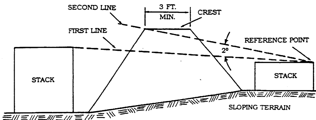
Figure C4.F2. Determination of Barricade Height (Sloping Terrain).
