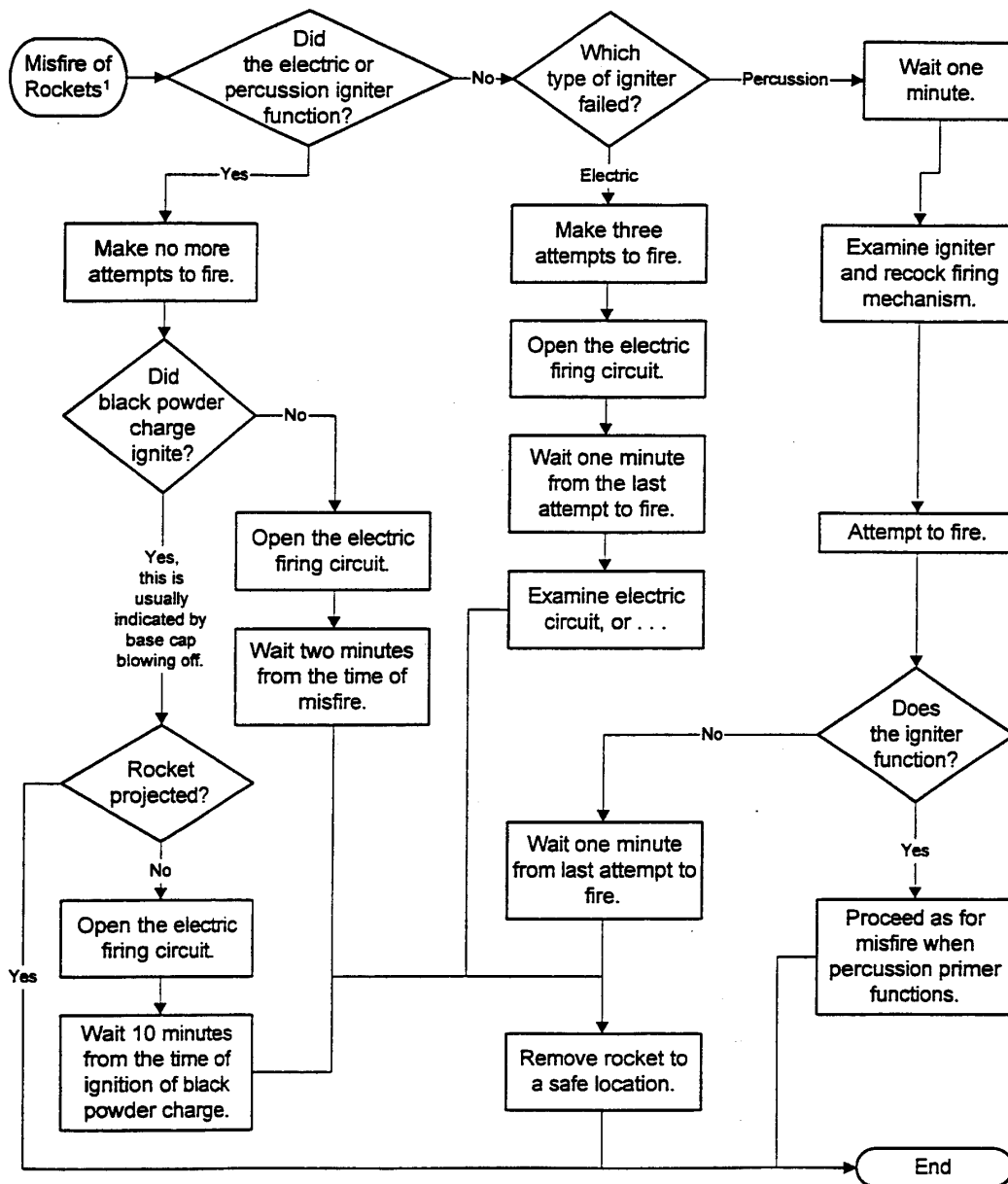
Figure C14.F7. Misfire of Rockets.
