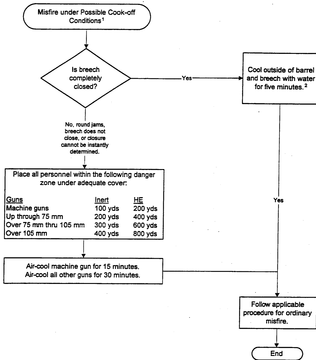
Figure C14.F4. Misfire Under Possible Cook-off Conditions.
