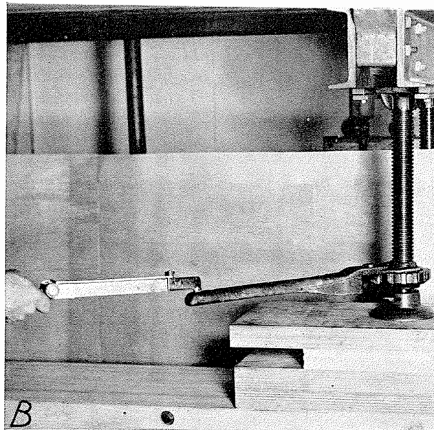
Figure 5-15. Instruments used in measuring loads applied by jackscrews; A, compressometer; B, torque wrench.
