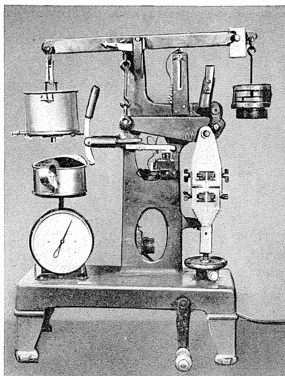
Figure 4-6. Plywood joint test: Test specimens and grips; testing machine.
