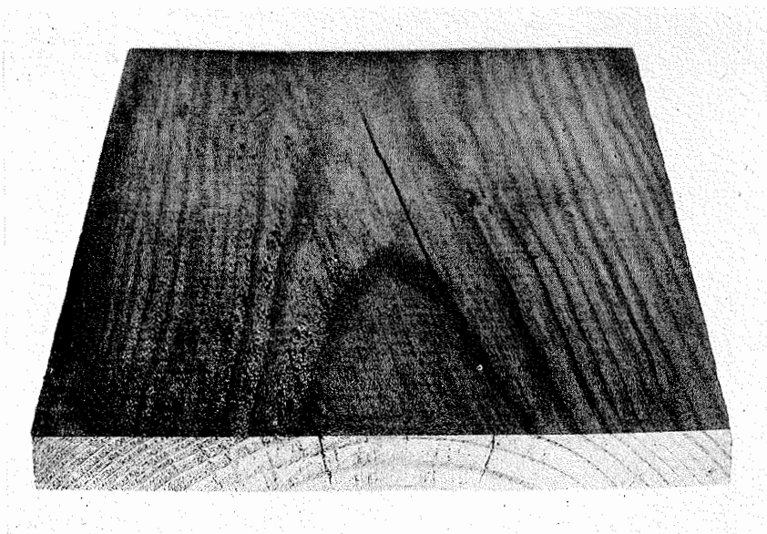
Figure 2-60. Checks in a flat-grain board.
