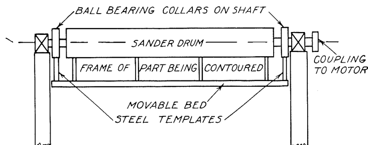
Figure 5-87. Contour drum sander for aircraft frame work.
