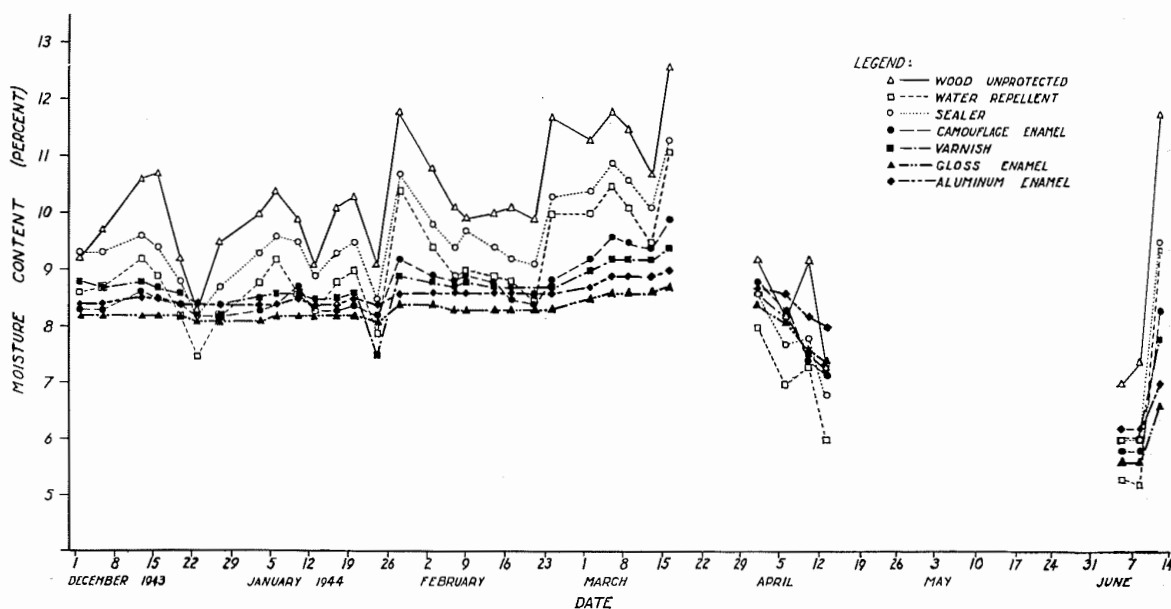
Figure 5-97. Variations in moisture content of three-ply, \frac{3}{32} -inch birch aircraft plywood kept in the air space within a naval glider wing mounted at Madison, Wis., from December 1943 to June 1944. As indicated by the legend, there were samples of plywood left unfinished and samples protected by each of the finishes described in detail in the title of figure 5-96.
