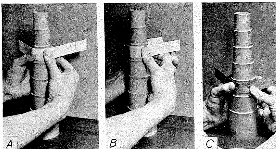
Figure 2-97. Mandrel bending test of veneer: A, start of test; B, finish of test; C, specimen showing breakage in the part with excessive slope of grain near the top but not in the remainder, which had permissible slopes.
