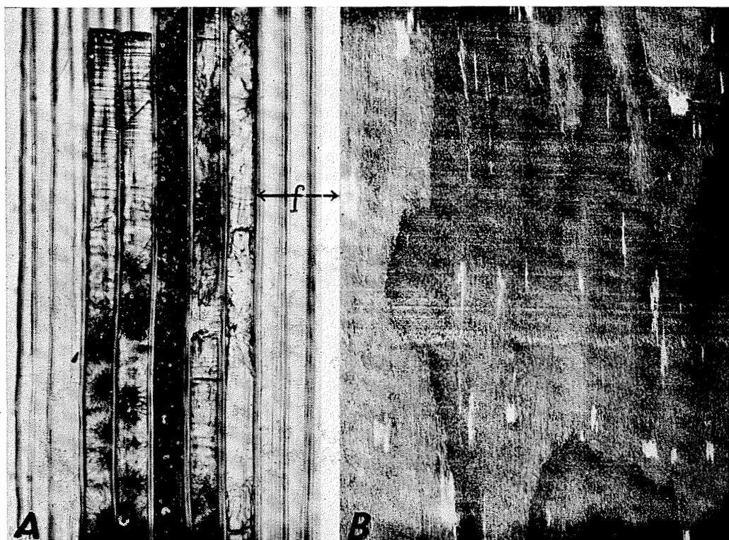
Figure 2-87. Floccosoids—white spots in western hemlock. A, floccosoids ( f ) as seen through the microscope (about 200X magnification); B, floccosoids ( f ) in rotary-cut veneer.
