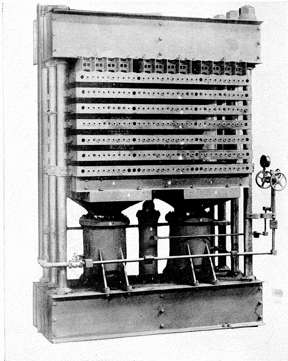
Figure 5-13. Hydraulic, 6-opening, hot-plate press used in the manufacture of flat plywood.
