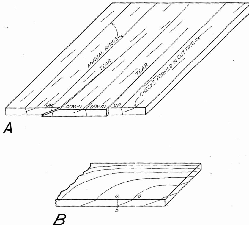
Figure 2-95. A, effect of checks formed in cutting on direction of tear in quarter-sliced veneer. B, method of measuring slope of grain through a sheet of veneer. The line bo represents the direction of the grain through the sheet as indicated by annual rings, pores, fibers, fracture, etc. The line ab represents the thickness of the veneer. Slope of grain equals ab/ao .
