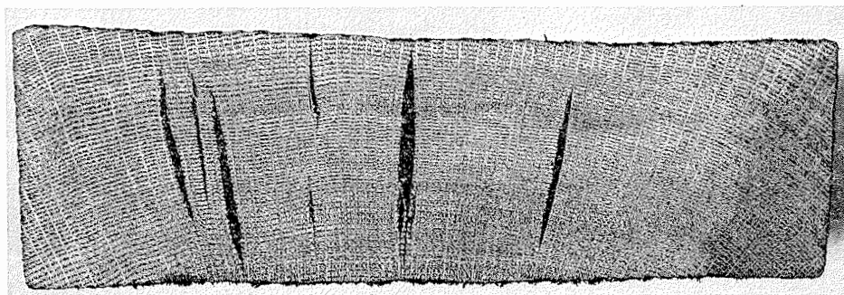
Figure 5-4. End of oak plank showing honeycombing.
