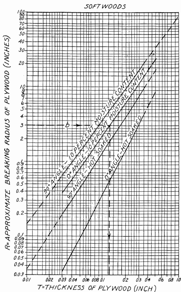
Figure 5-90. Approximate relation between thickness and breaking radius in the bending of softwood plywood. Softwoods tested were Douglas-fir, Sitka spruce, and western white pine. (For explanation of this graph, see sec. 5.6830.)
