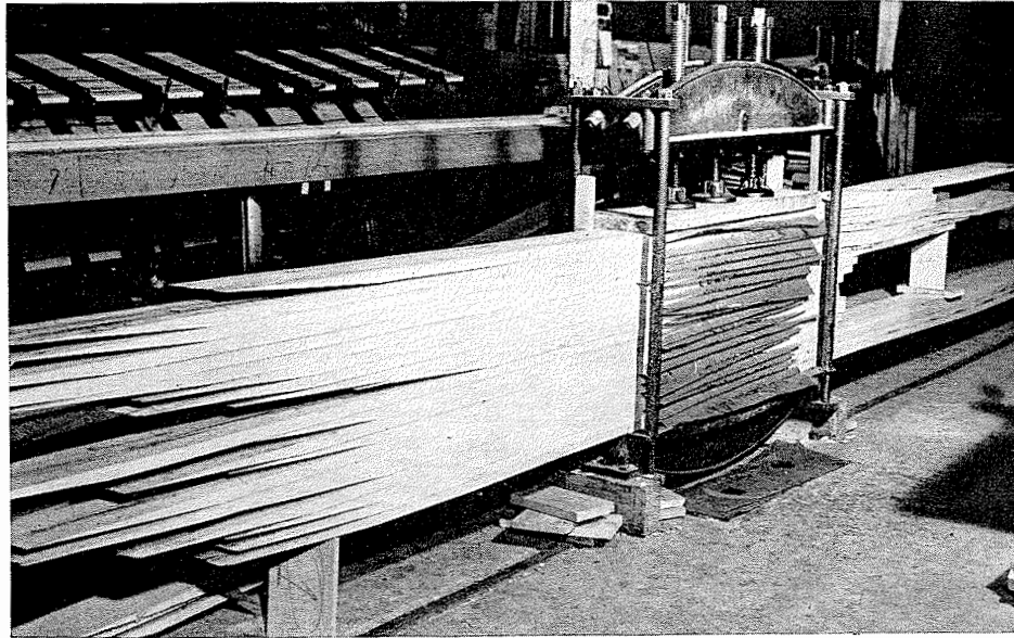
Figure 5-36. Screw press used in gluing scarf joints. In presses of this type some provision should be made to prevent end slippage (sec 5.4100).
