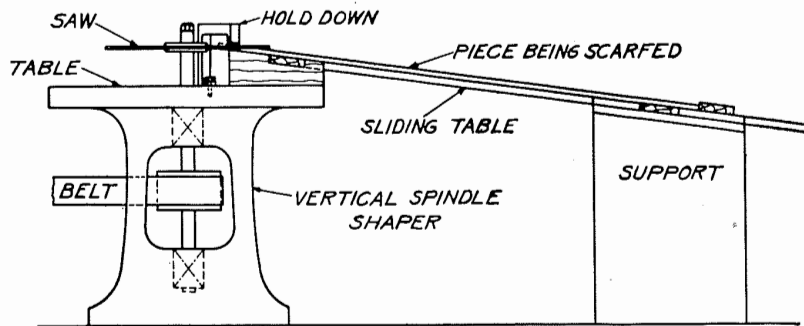
Figure 5-74. Special saw-scarfing machines. Plywood is held rigidly in position on table by hold-down. Scarf is cut by moving table past saw (A), or by moving saw past table (B). Tilt of saw or table determines slope of scarf.
