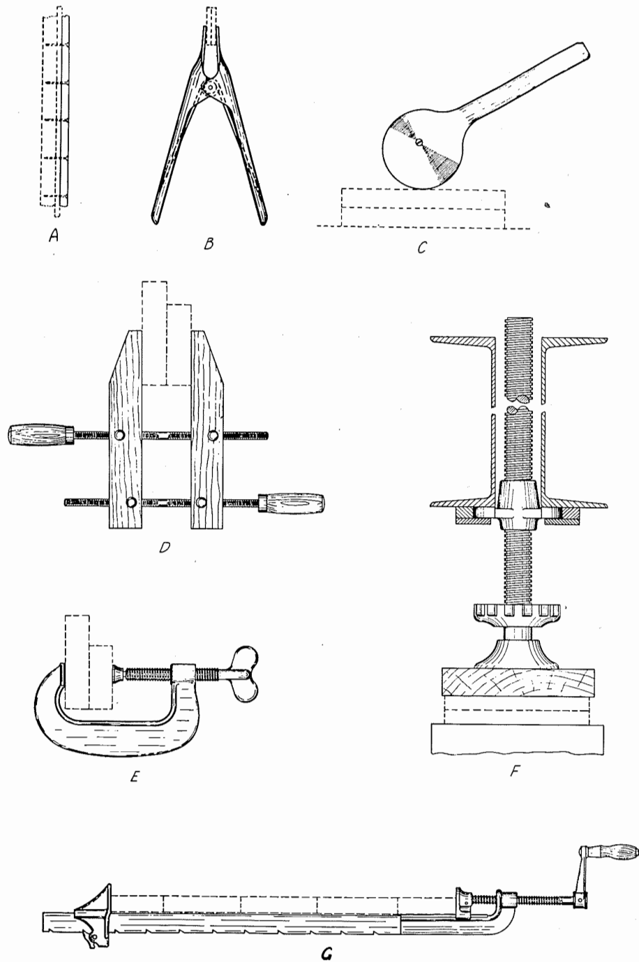
Figure 5-14. Hand devices used in applying pressure to glue joints; A, brads, screws, or nails; B, spring clamp; C, eccentric clamp; D, wood clamp; E, C-clamp; F, jackscrews; G, bar clamp.
