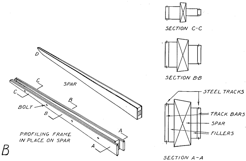
Figure 5-82. Spar profiling: A, profiling machine in operation; B, details of frame employed for profiling and beveling spars by moving spar past a stationary jointer.
