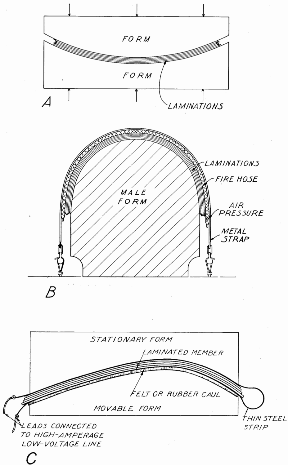
Figure 5-39. Diagrams of apparatus used in gluing curved laminated members.
