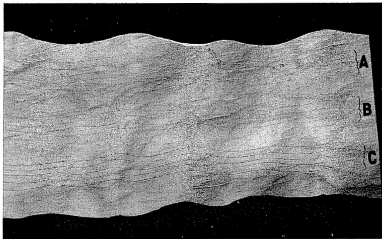
Figure 2-57. Tangential surface of wood tested with scribes to determine direction of grain. Note parallelism of scribe marks in same areas.
