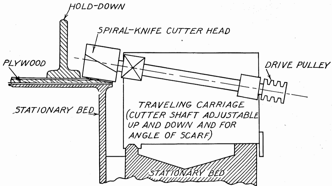
Figure 5-73. Traveling cutter-head scarfing machine.
