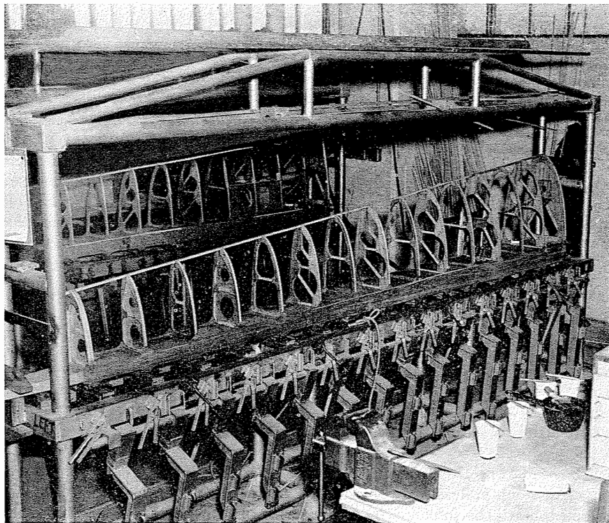
Figure 5-51. Jigs for locating leading-edge ribs in proper positions.
