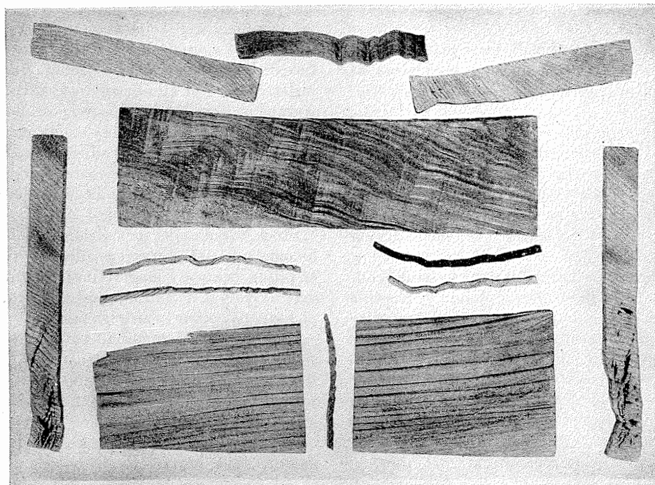
Figure 5-5. Collapse in western red cedar.
