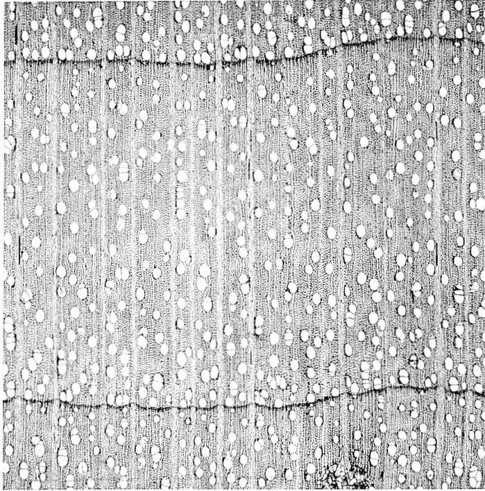
Figure 2-21. Red maple. Cross section magnified 20 diameters. Pill fleck in lower right-hand quarter.
