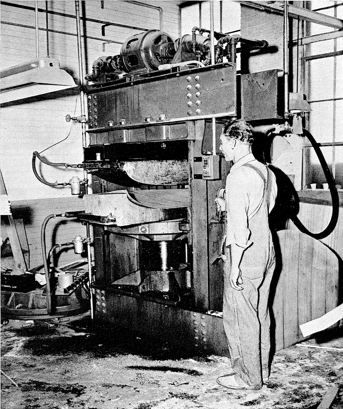
Figure 5-92. Bending flat plywood to desired shape between heated plates.
