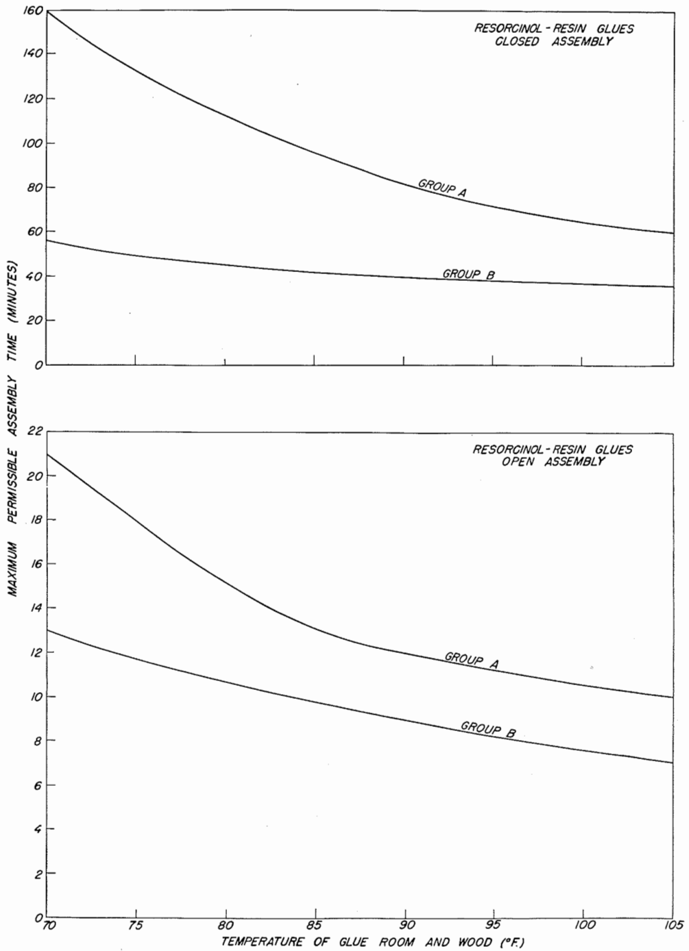
Figure 5-19. Effect of temperature upon maximum closed and open assembly periods for resorcinol-resin glues. (Curves based on single spread of glue at the expiration of 75 percent of its working life.)
