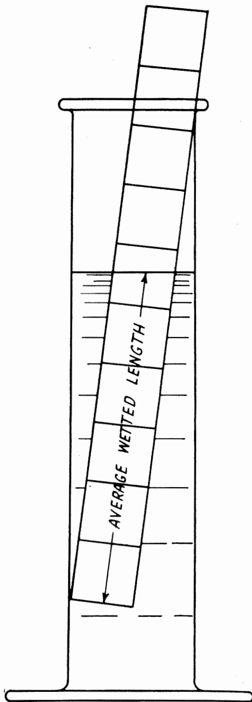
Figure 2-44. Flotation method of determining specific gravity or unit weight. The operation may be expedited and the accuracy enhanced if the vessel is filled to overflowing and the water line marked on the specimen immediately after immersion.
