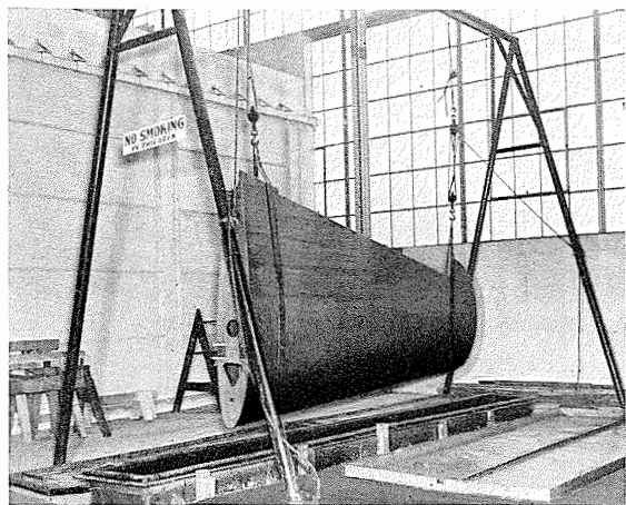
Figure 5-101. Dipping tank set in floor of finishing room holding about 2,000 gallons of varnish sealer in which plywood-covered wing sections are dipped twice to finish all interior surfaces and seal the outside surfaces.
