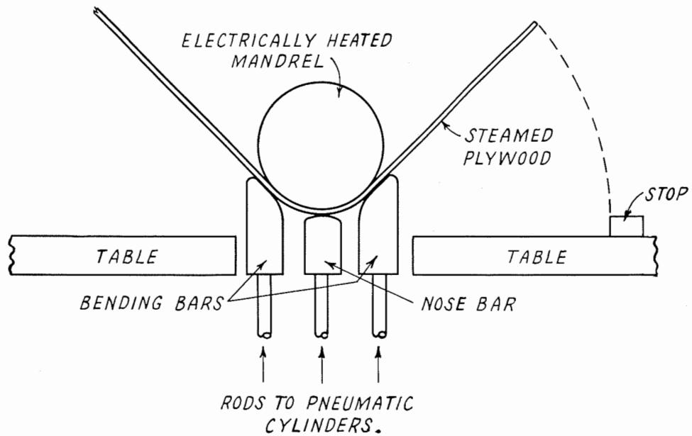
Figure 5-94. Cross section of steam-bending machine.
