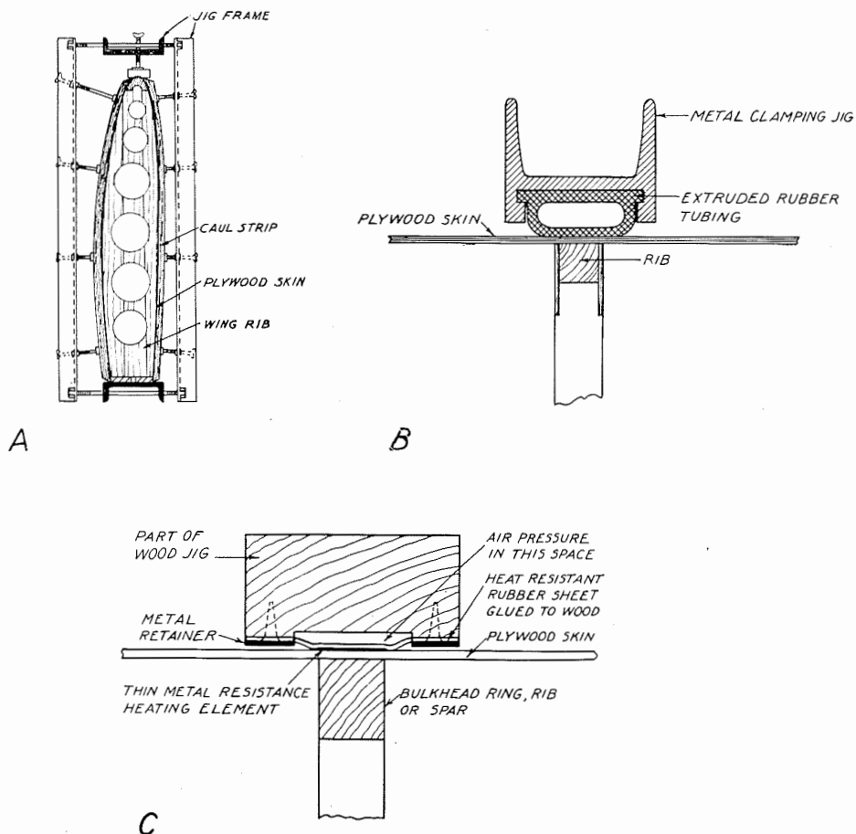
Figure 5-62. Devices for applying gluing pressure and heat in covering wings.
