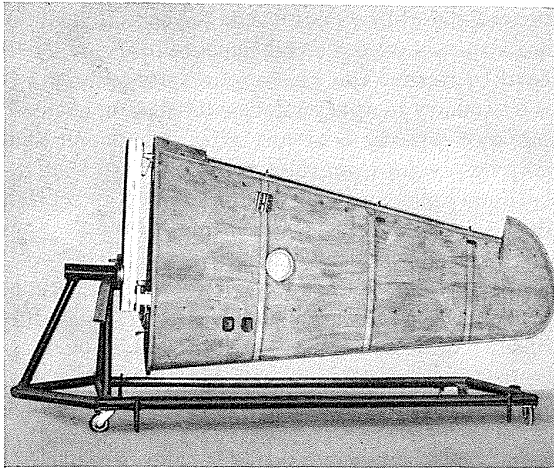
Figure 5-104. Fabric-covered wing section after applying clear dope. The clear dope contains a little blue dye for identification in the factory. Note the dolly on which the wing section is moved through the various steps in finishing.
