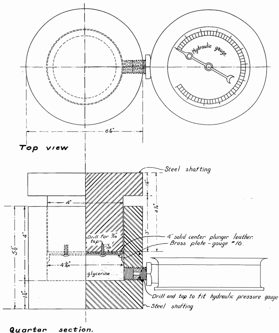
Figure 5-16. Detailed drawing of compressometer; used to measure loads applied by jackscrews.
