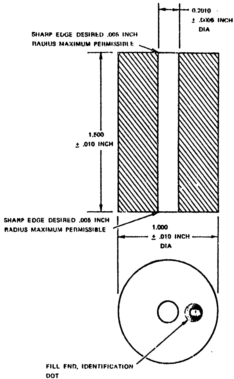
FIG. 3-4. Body.
