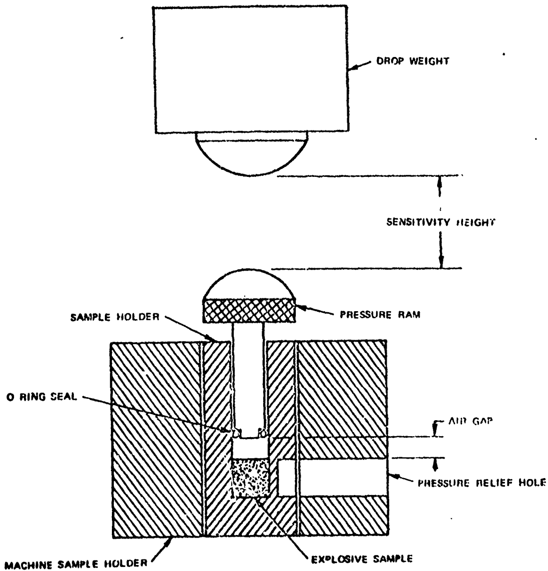
FIG. 8-1. Adiabatic Sensitivity Test Machine.
