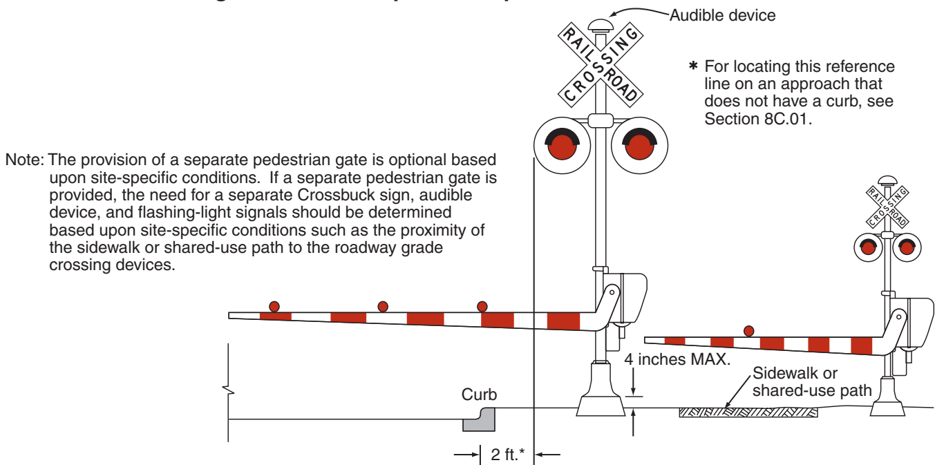
Figure 8C-6. Example of a Separate Pedestrian Gate
