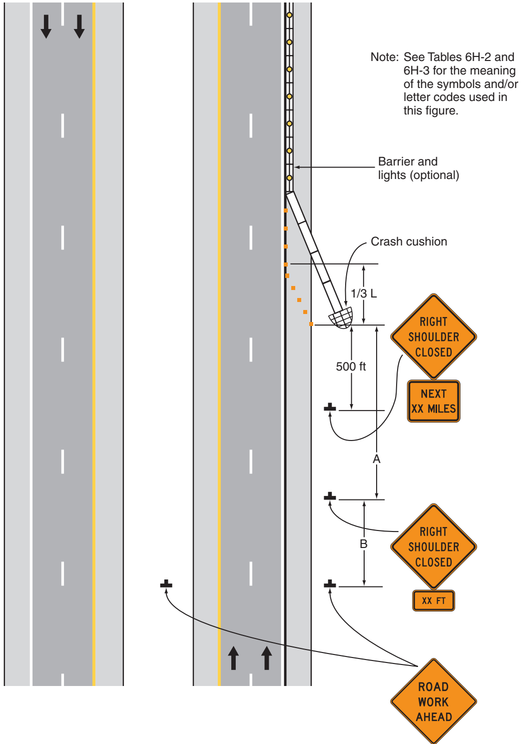
Typical Application 5
