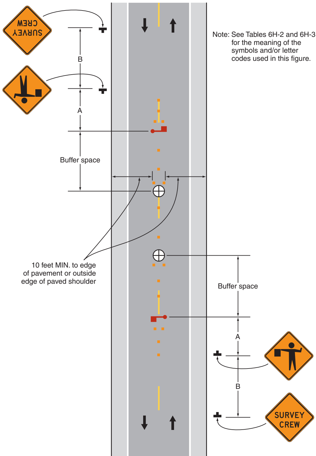
Typical Application 16
