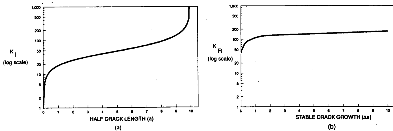
Figure 2-26. K_I and K_R curves (logarithmic scale)
