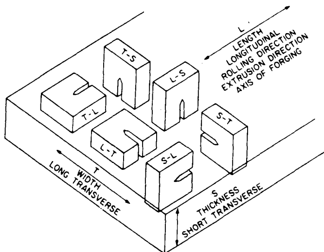
Figure 2-14. CTS orientation.
