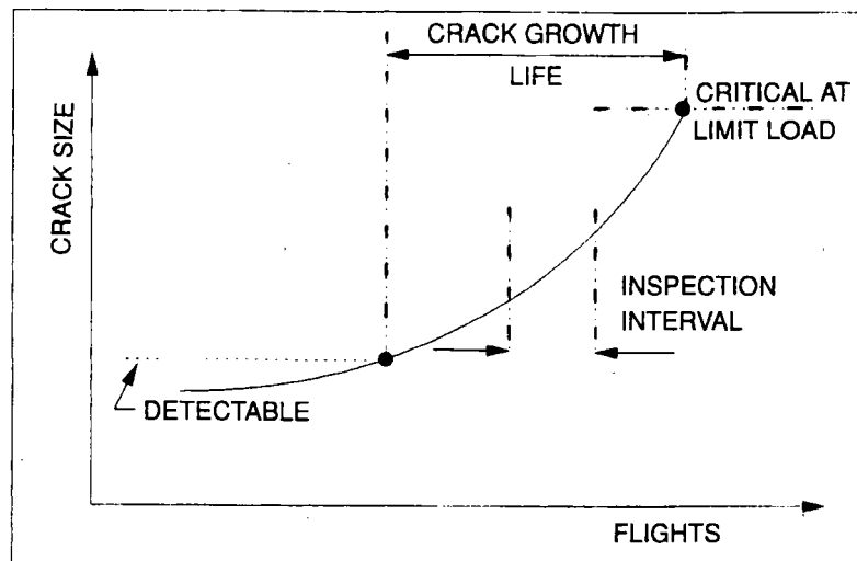
Figure 1-16. Crack growth in response to cyclic loads.
