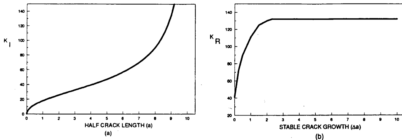
Figure 2-25. K_I and K_R curves
