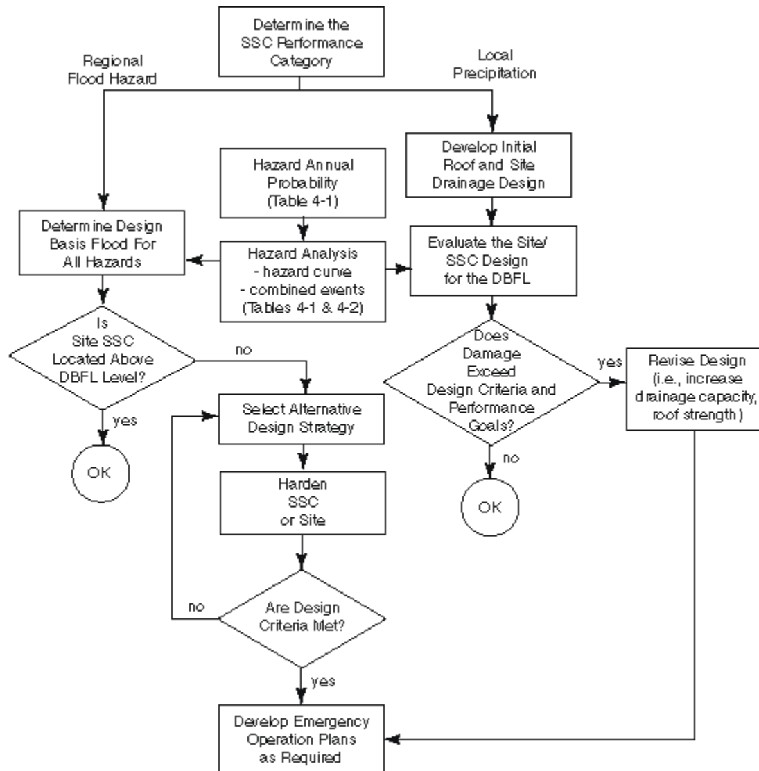
Figure 4-1 Flood Evaluation Process
