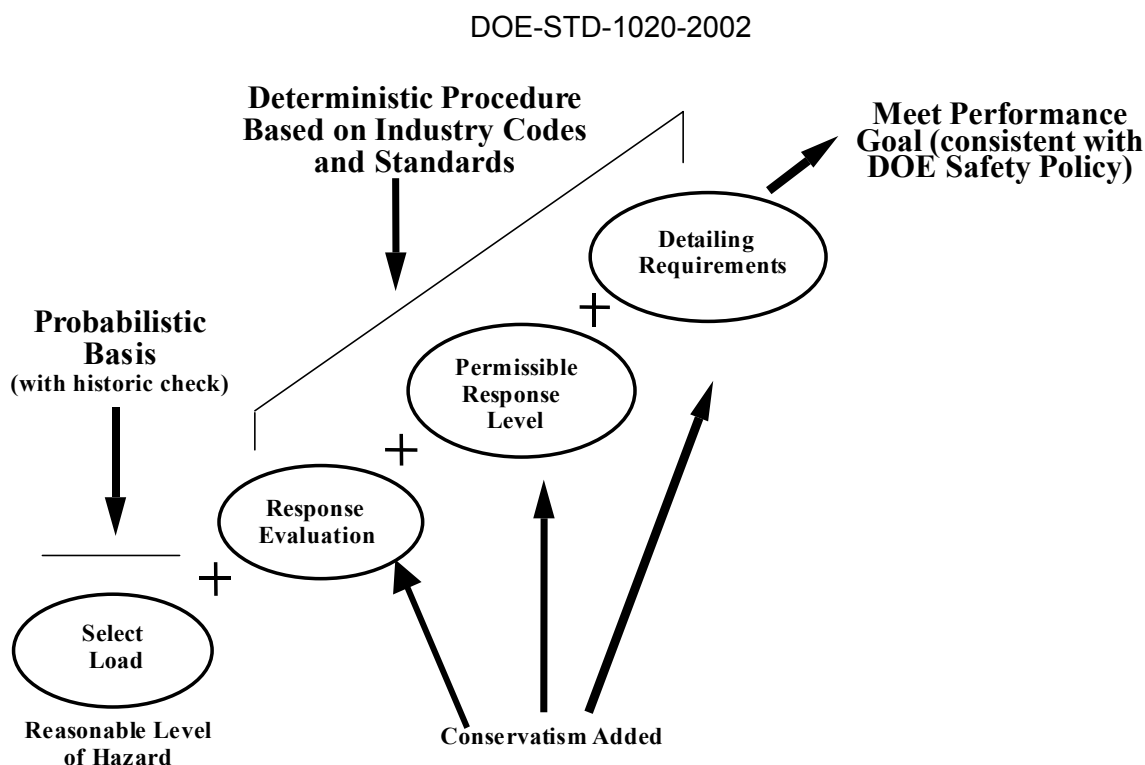
Figure 2-1. DOE-STD-1020 Combines Probabilistic and Deterministic Methods to Achieve Performance Goals
