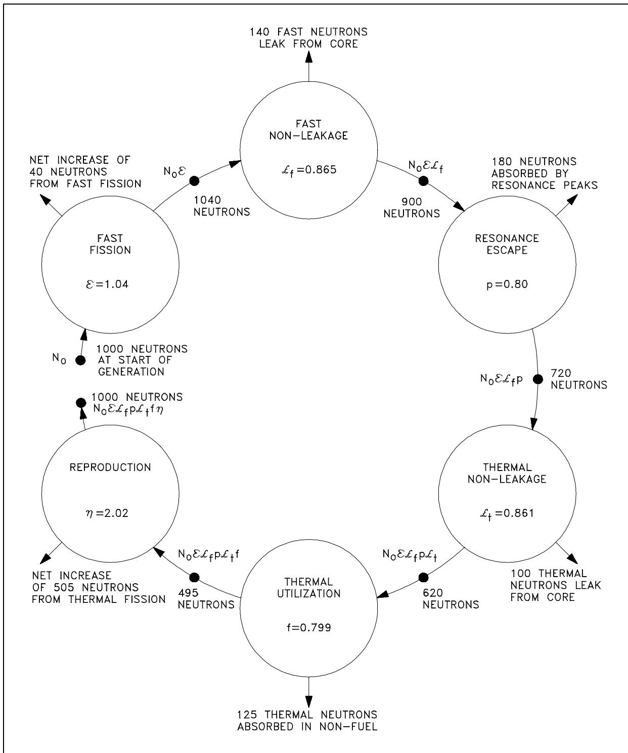
Figure 1 Neutron Life Cycle with k_{\text{eff}} = 1
