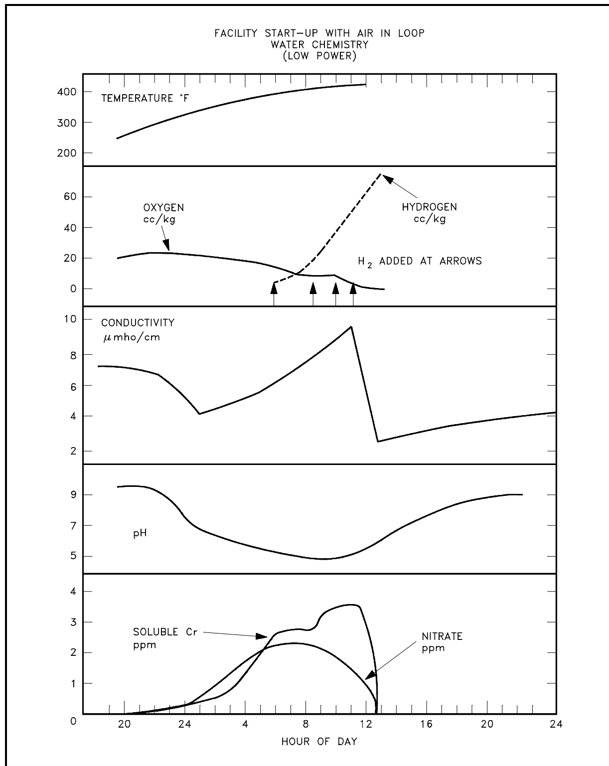
Figure 6 Facility Start-up With Air in Loop
