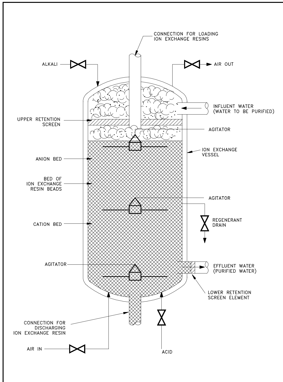
Figure 3 Schematic Diagram of a Typical Ion Exchanger
