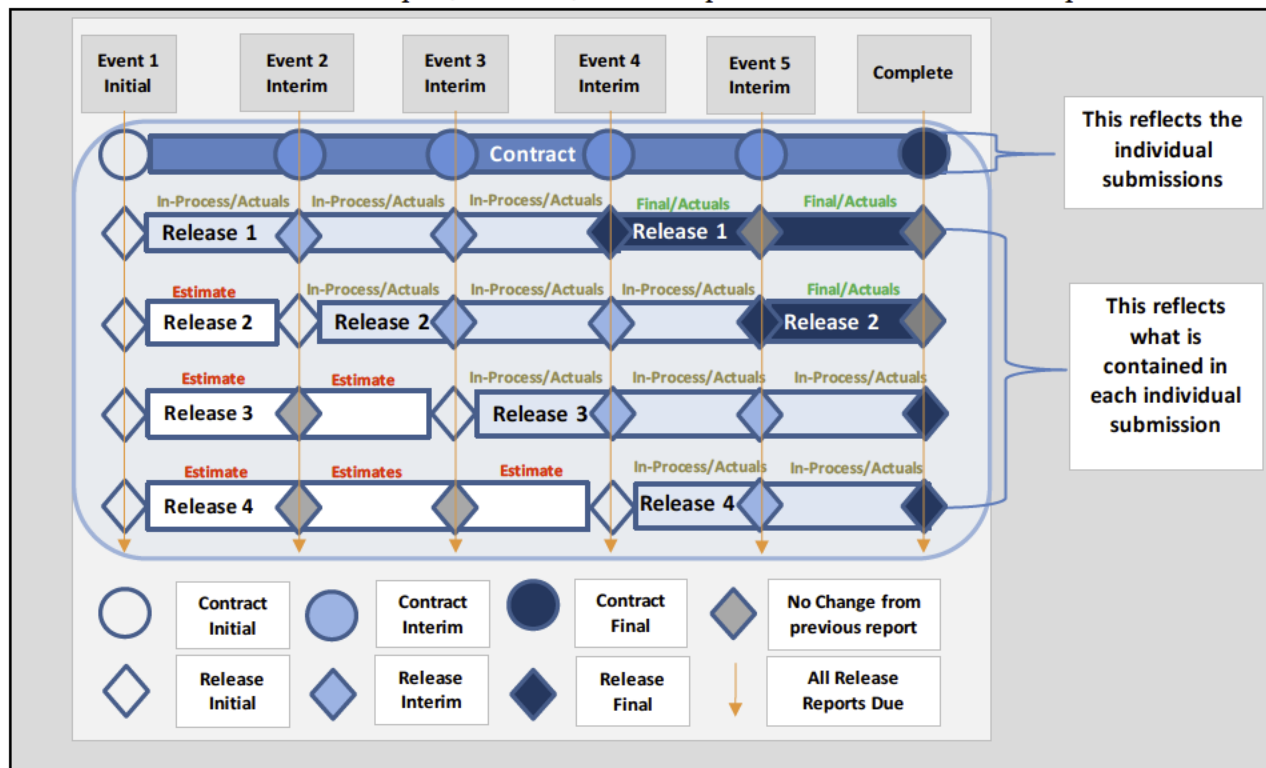
Figure 1: Software Development Reporting Process
