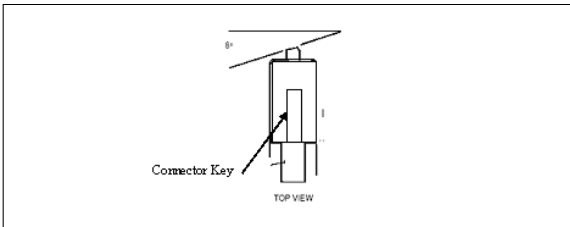
FIGURE 2. SC APC ferrule/angle orientation.
