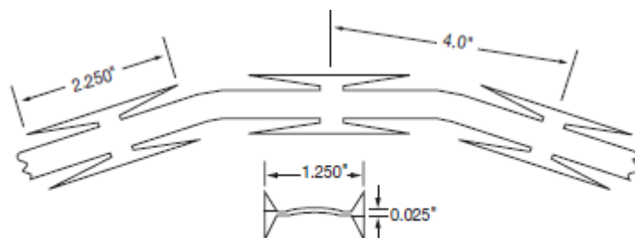
FIGURE 1. BARBED TAPE.
