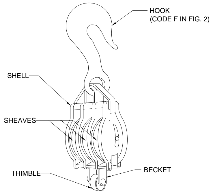
Figure 1. Block with hood fitting.
