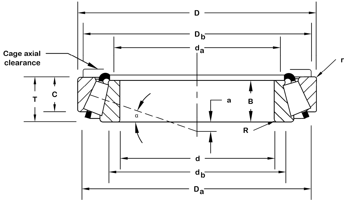
FIGURE 1. Bearing characteristics.
