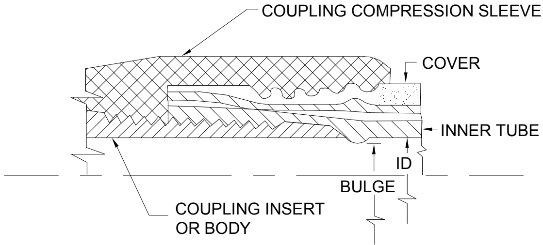
FIGURE 1. Hose dimensions.
