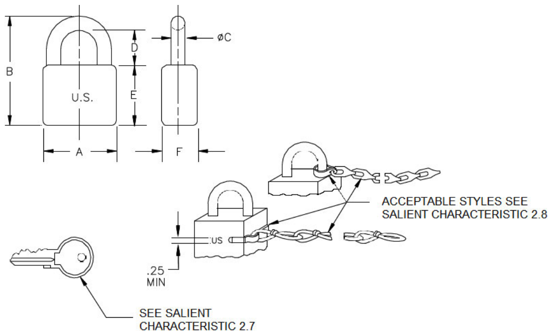
FIGURE 1. PADLOCK.
