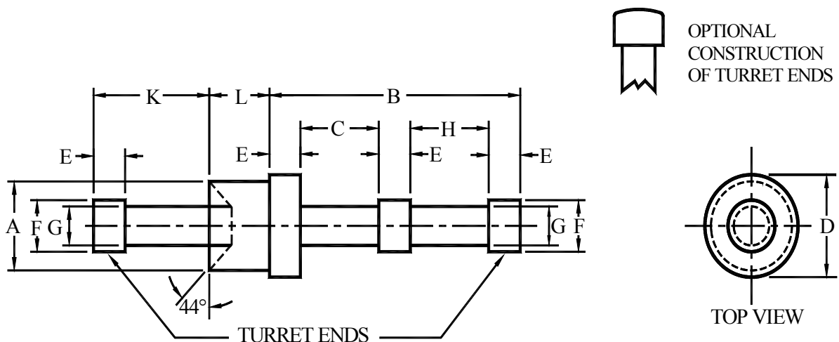
Figure 1. Single double feedthru stud terminal .
