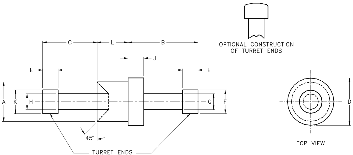
FIGURE 1. Single feedthru terminal stud.
