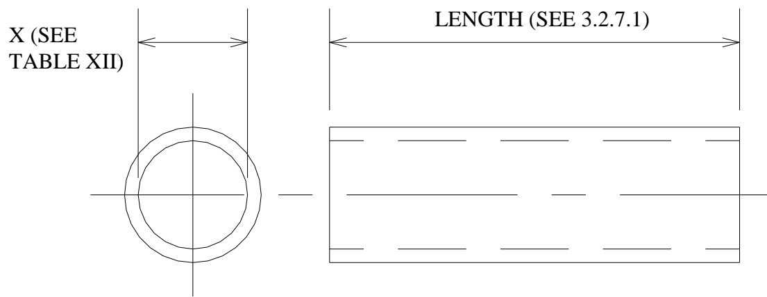
FIGURE 1. Type I hose.
