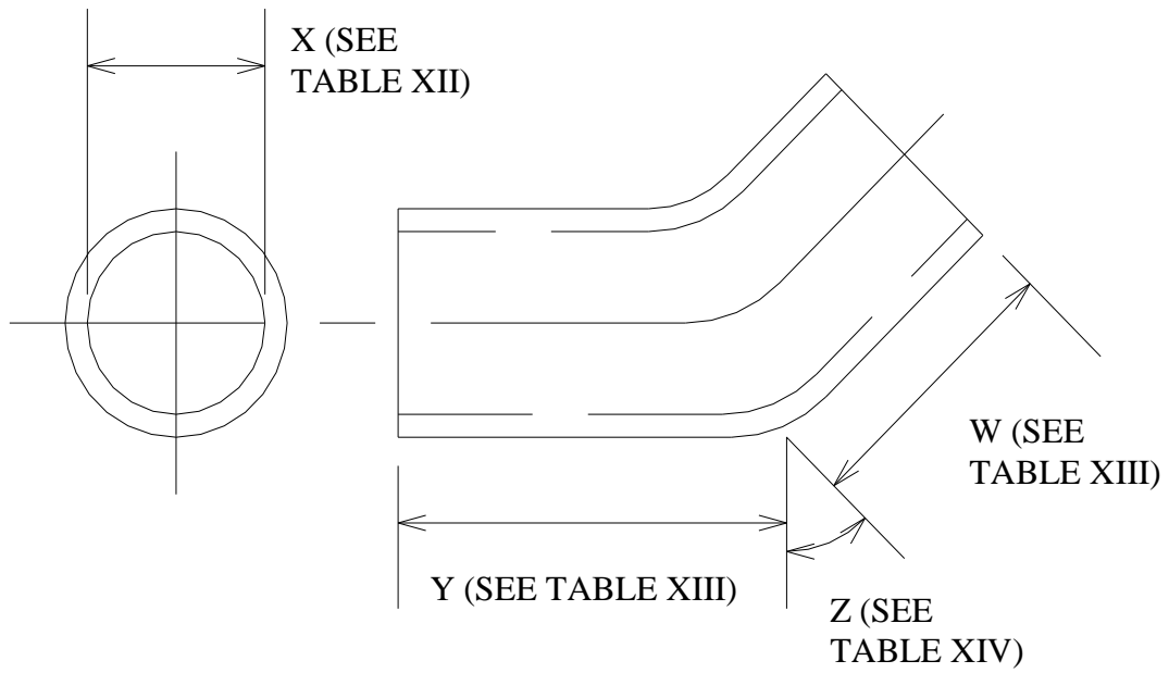
FIGURE 2. Type II hose.
