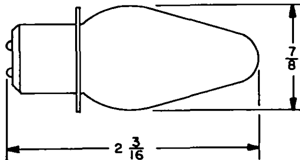
FIGURE 1. Lamp dimensions (inches).
