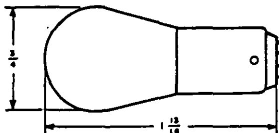
FIGURE 1. Lamp dimensions (inches).
