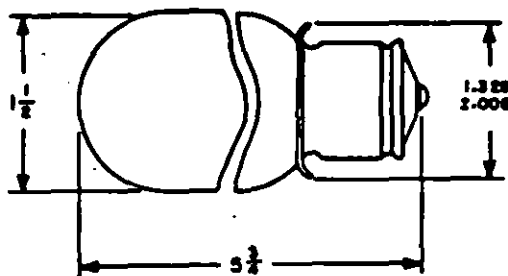
FIGURE 1. Lamp dimensions (inches).
