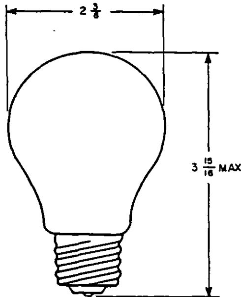
FIGURE 1. Lamp dimensions (inches).
