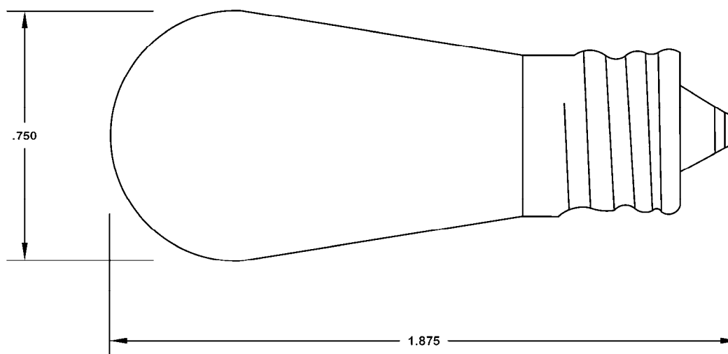
FIGURE 1. Lamp dimensions (inches).
