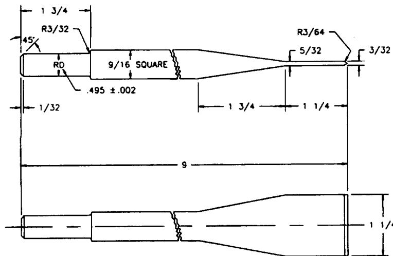
Figure 1. Chisel, scaling, power hammer.
