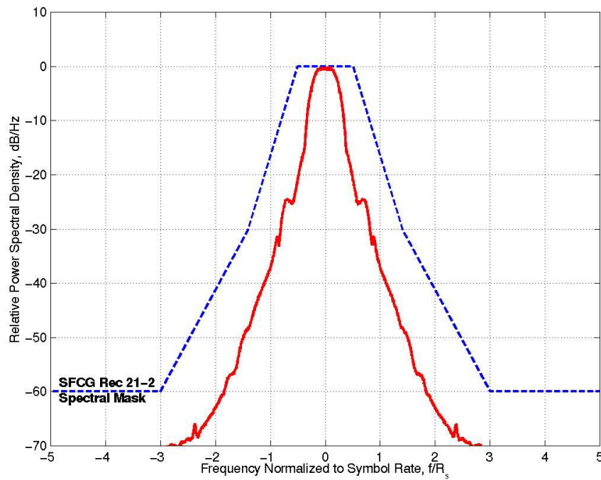
Figure 3-32: Simulated Spectrum of Nyquist Pulse-Shaped SRRC ( \alpha=0.5 ) OQPSK at Output of Saturated SSPA
