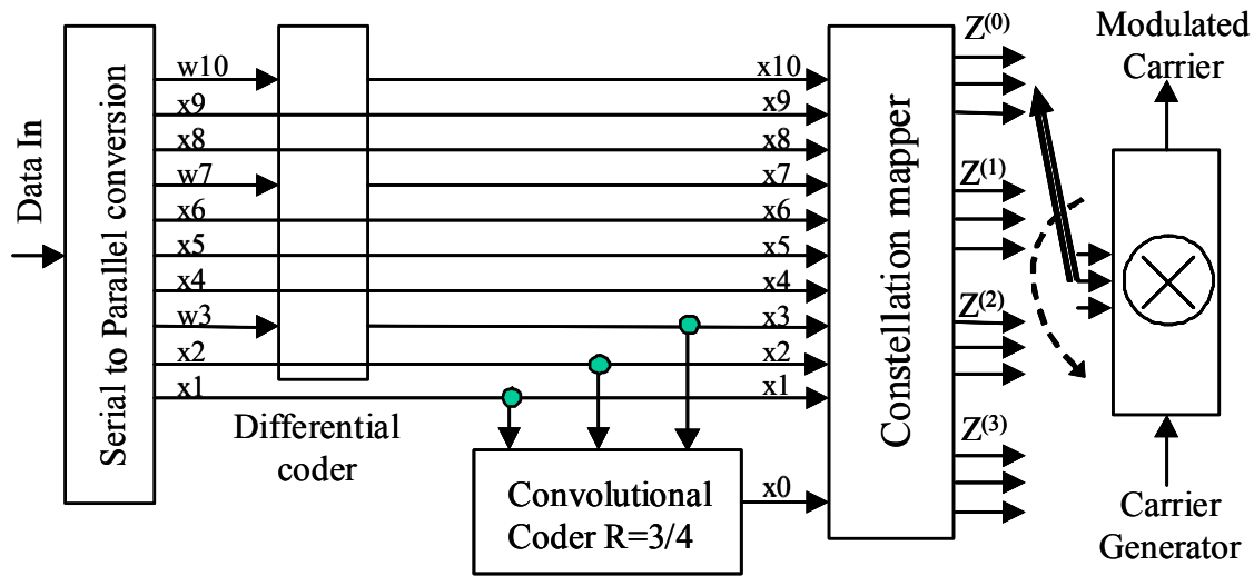
Figure 3-52: Coder and Mapper Implementation at 2.5 Bits/Channel-Symbol Efficiency
