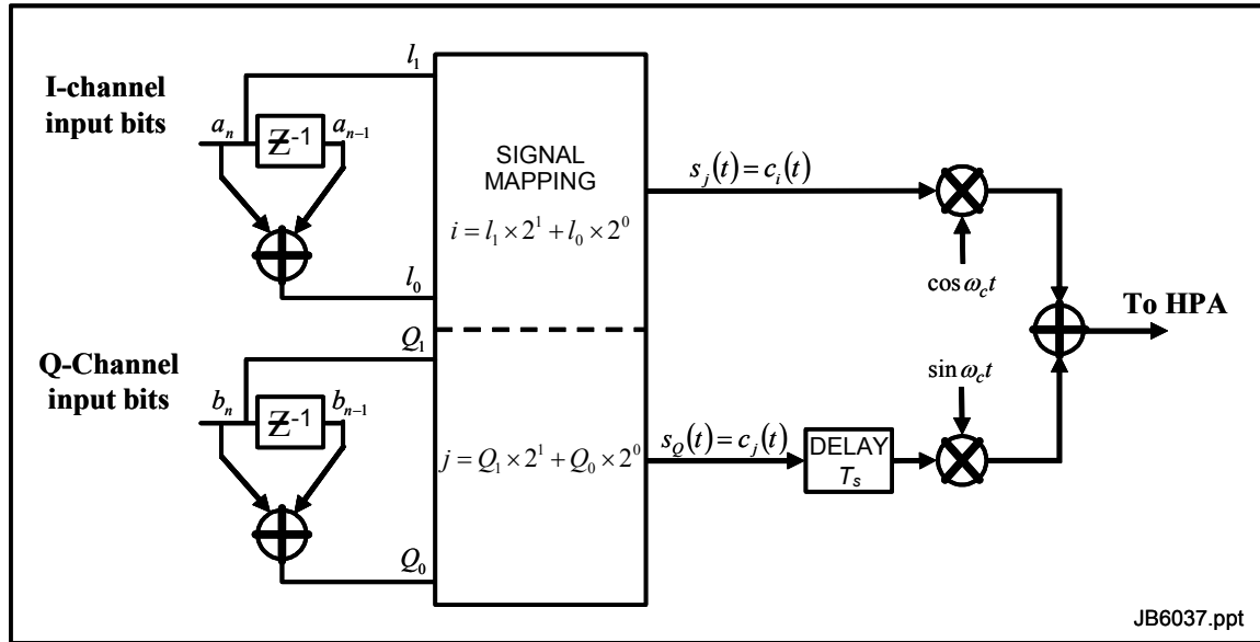
Figure 3-40: T-QPSK Modulator
