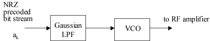
Figure 3-2: GMSK: Generated Using VCO
