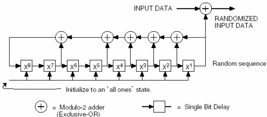
Figure 7-1: Logic Diagram for the Bit Transition Generator
